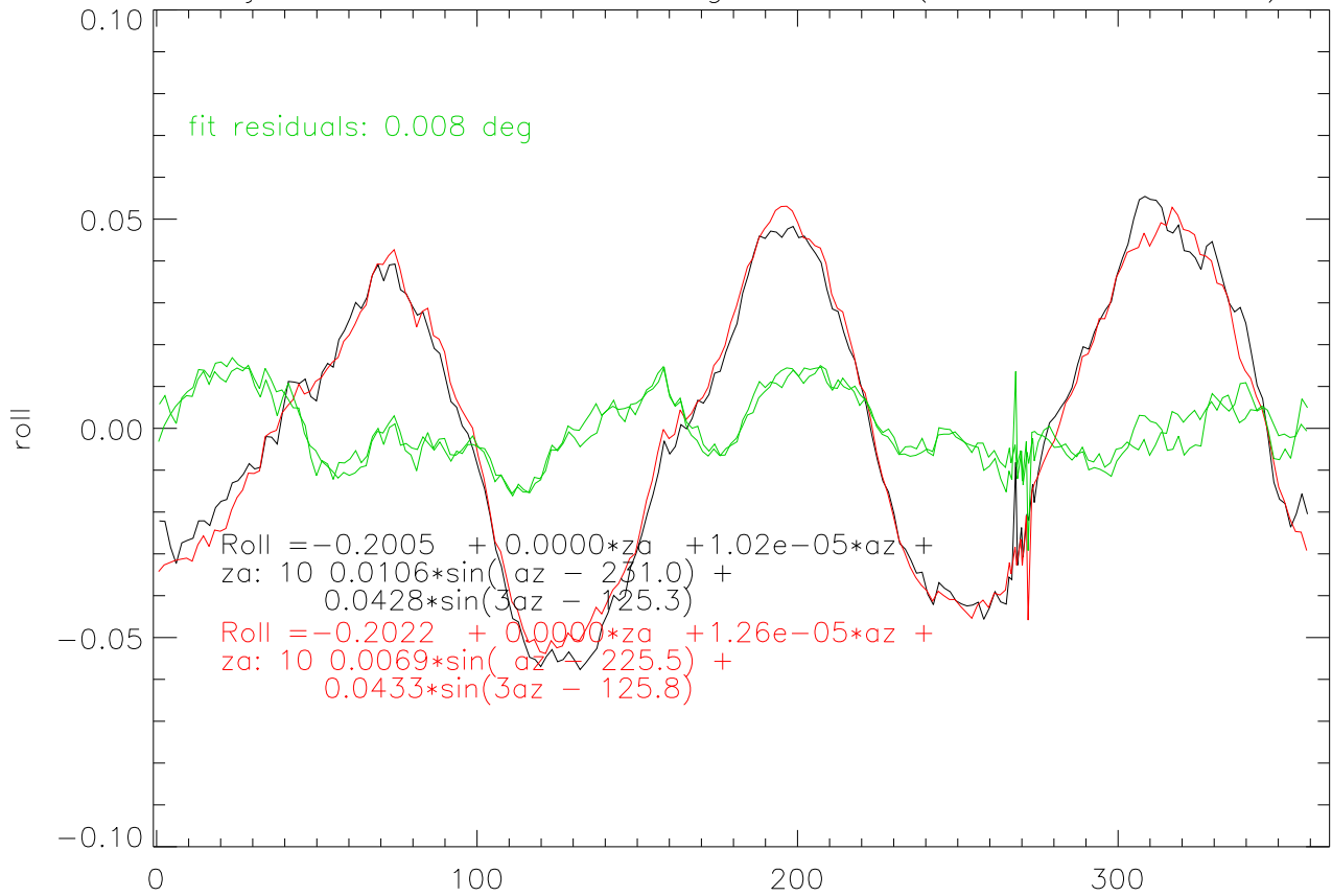
22jun11 tilt sensor az swings Roll - (c0+c1*az from fit)
