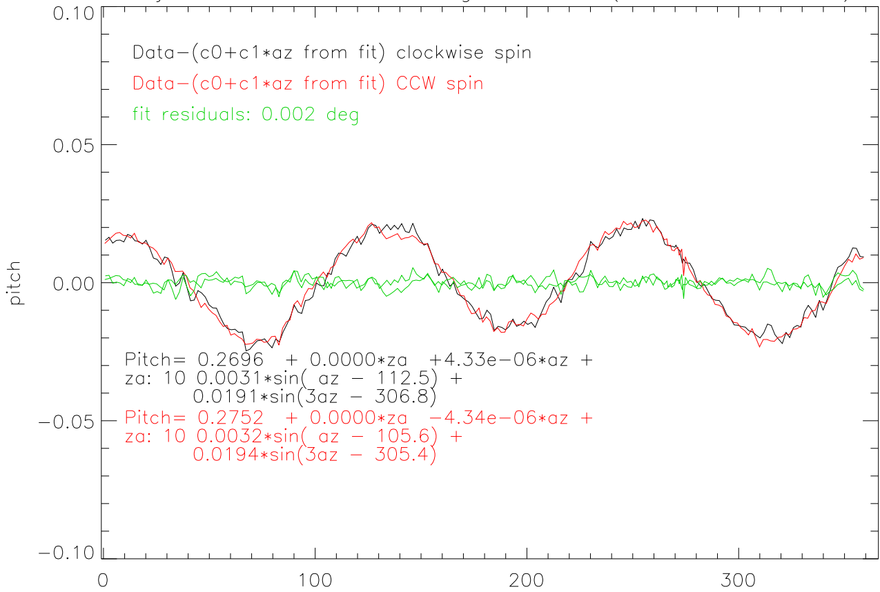
22jun11 tilt sensor az swings PITCH - (c0+c1*az from fit)
