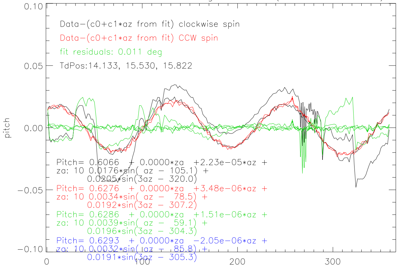
16feb12 tilt sensor az swings PITCH - (c0+c1*az from fit)
