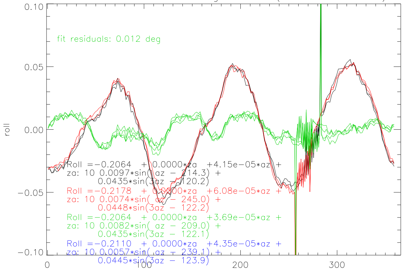
16feb12 tilt sensor az swings Roll - (c0+c1*az from fit)
