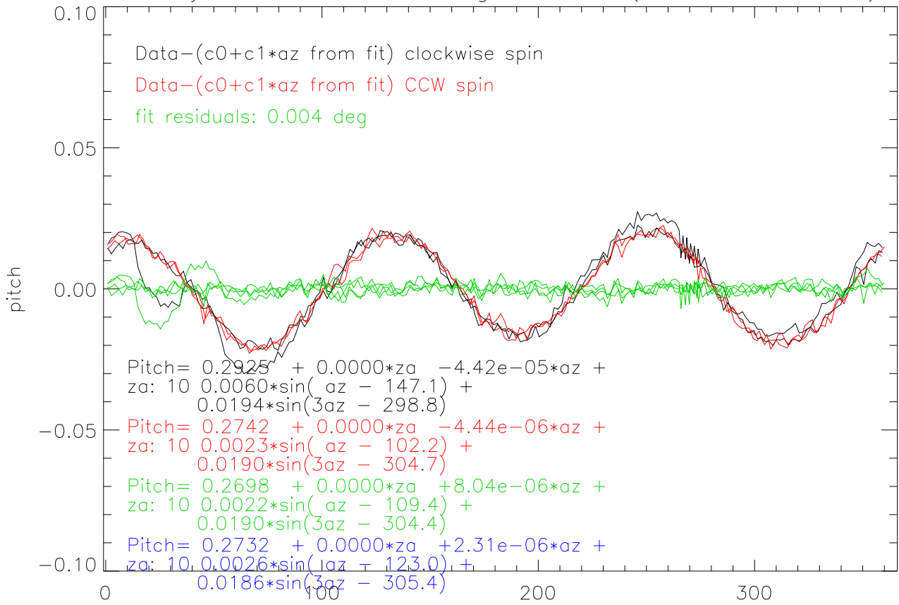
12may11 tilt sensor az swings PITCH - (c0+c1*az from fit)
