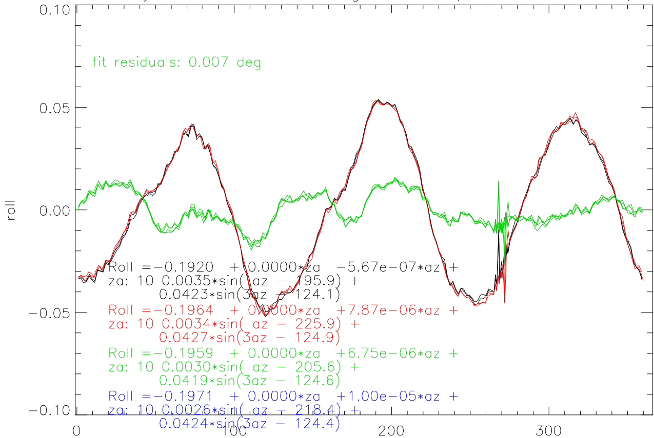
12may11 tilt sensor az swings Roll - (c0+c1*az from fit)
