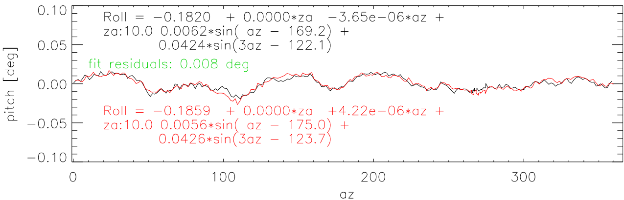
Residual from roll fit
