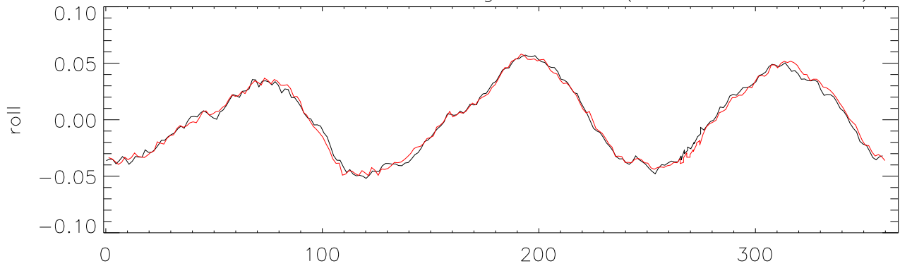
11mar14 tilt sensor az swings Roll - (c0+c1*az from fit)
