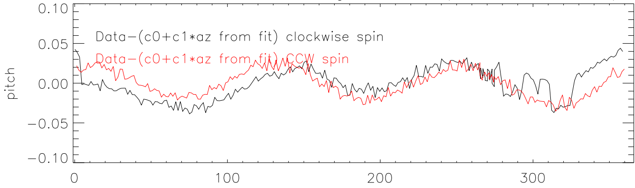
11mar14 tilt sensor az swings PITCH - (c0+c1*az from fit)
