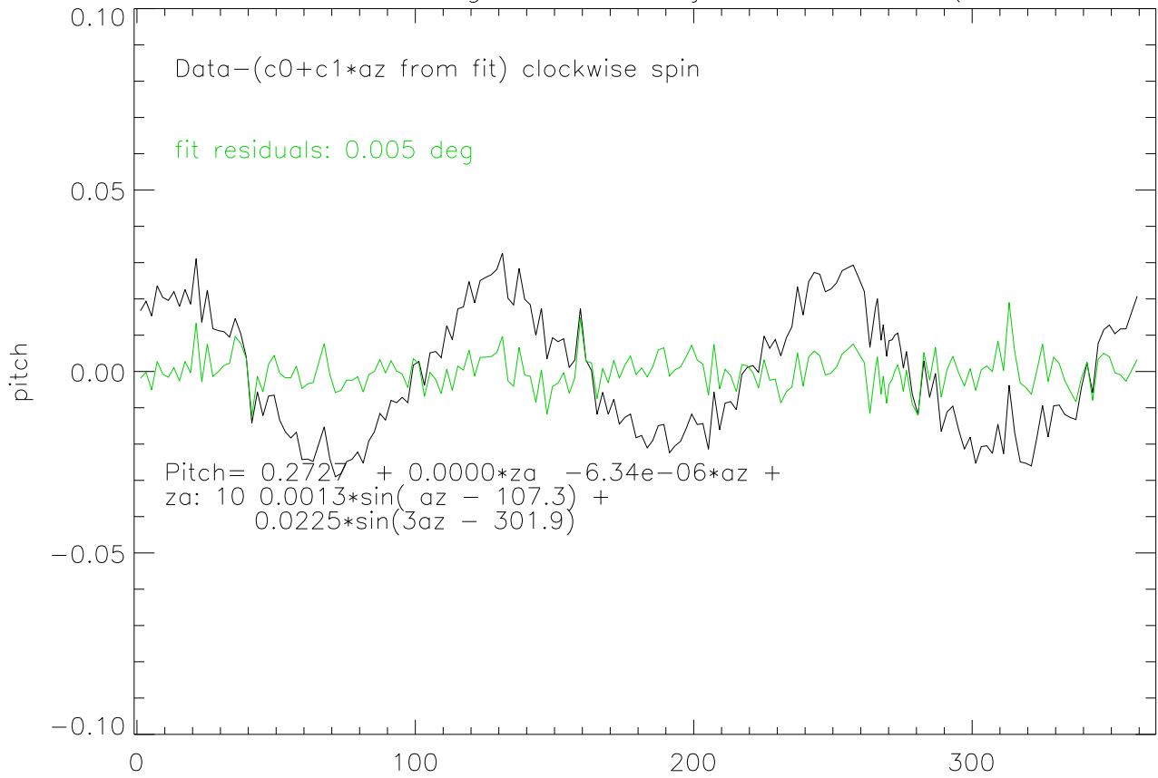
10dec07 tilt sensor az swings after td adjusted PITCH - (c0+c1*az from fit)
