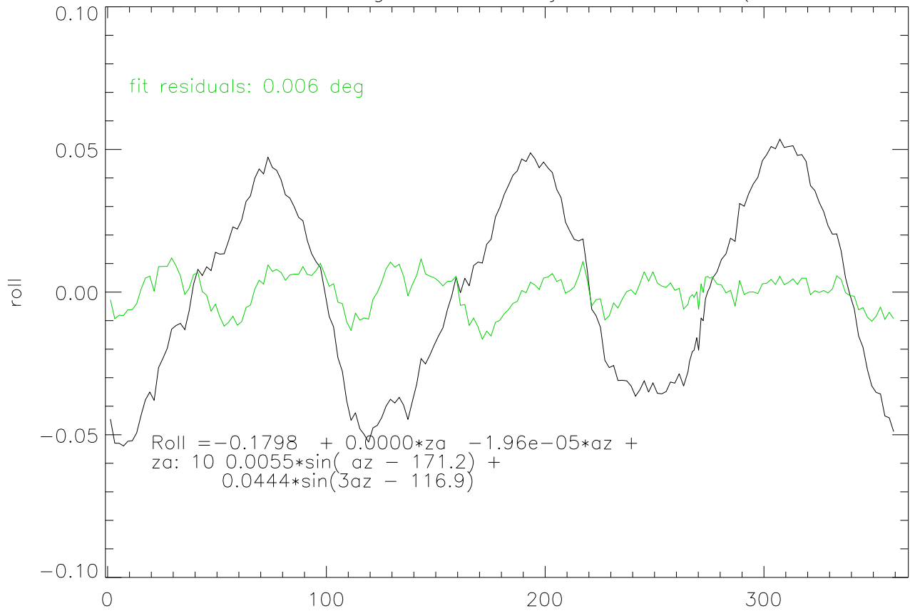
10dec07 tilt sensor az swings after td adjusted Roll - (c0+c1*az from fit)
