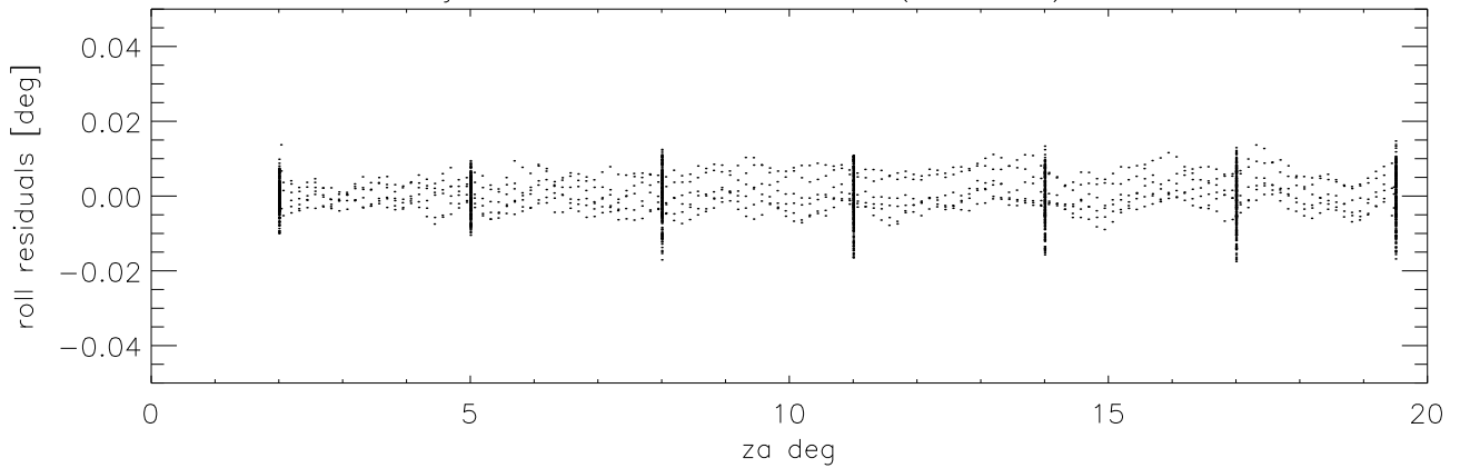
16jun12 2dfit roll residuals (data-fit) vs za
