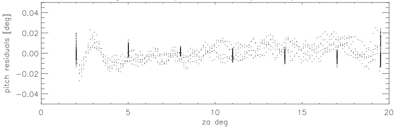
16jun12 2dfit roll residuals (data-fit) vs az
