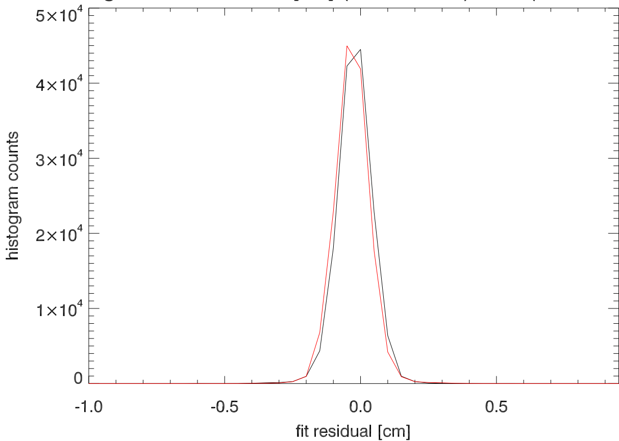
Histogram of fit residuals [cm] (measured-fit) 2014 (no zrotation)
