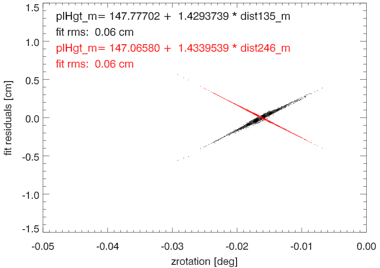
(2014-2015):fit residuals vs platform z axis rotation. no zrotation
