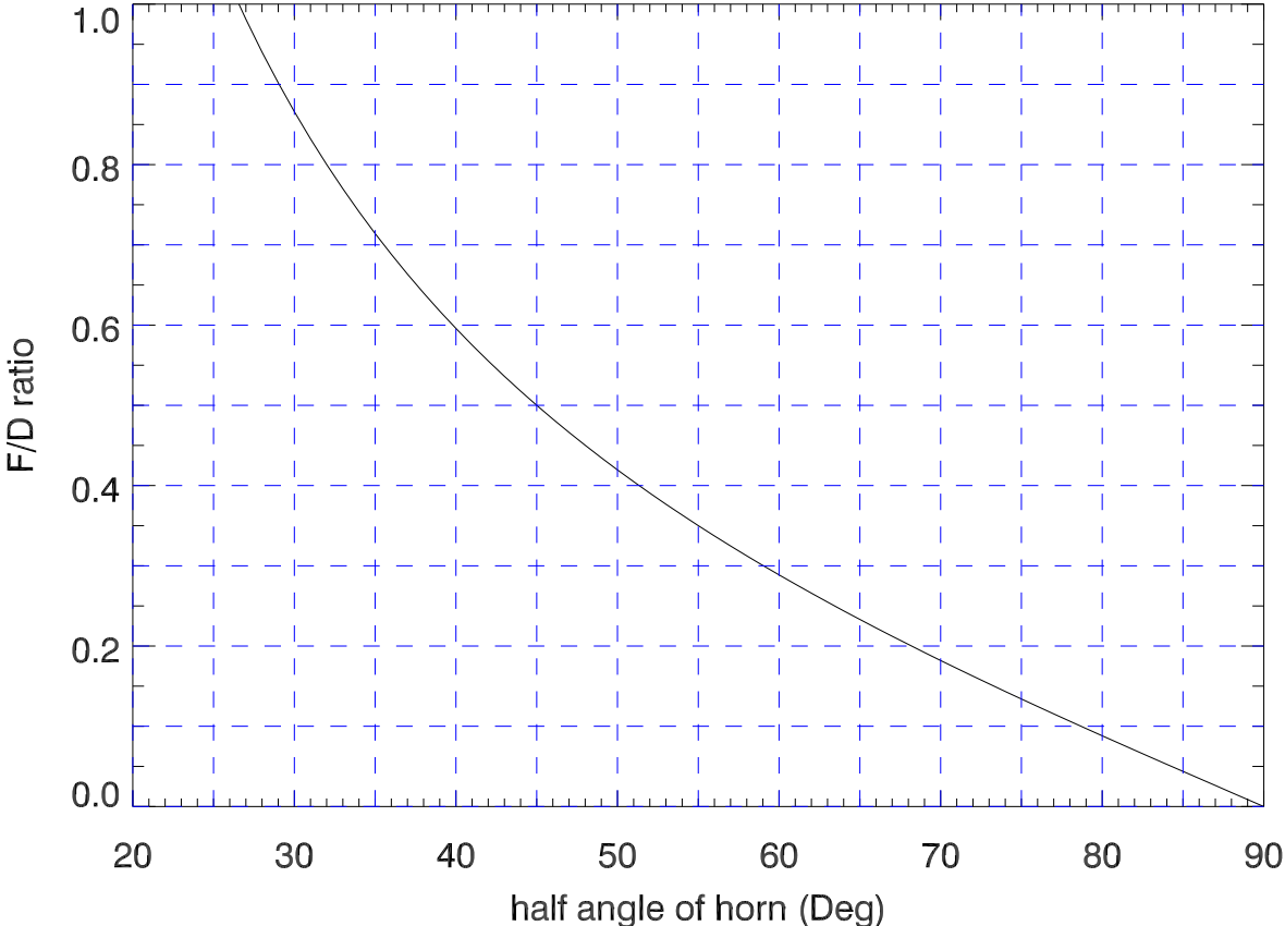
F over D ratio vs horn 1/2 angle
