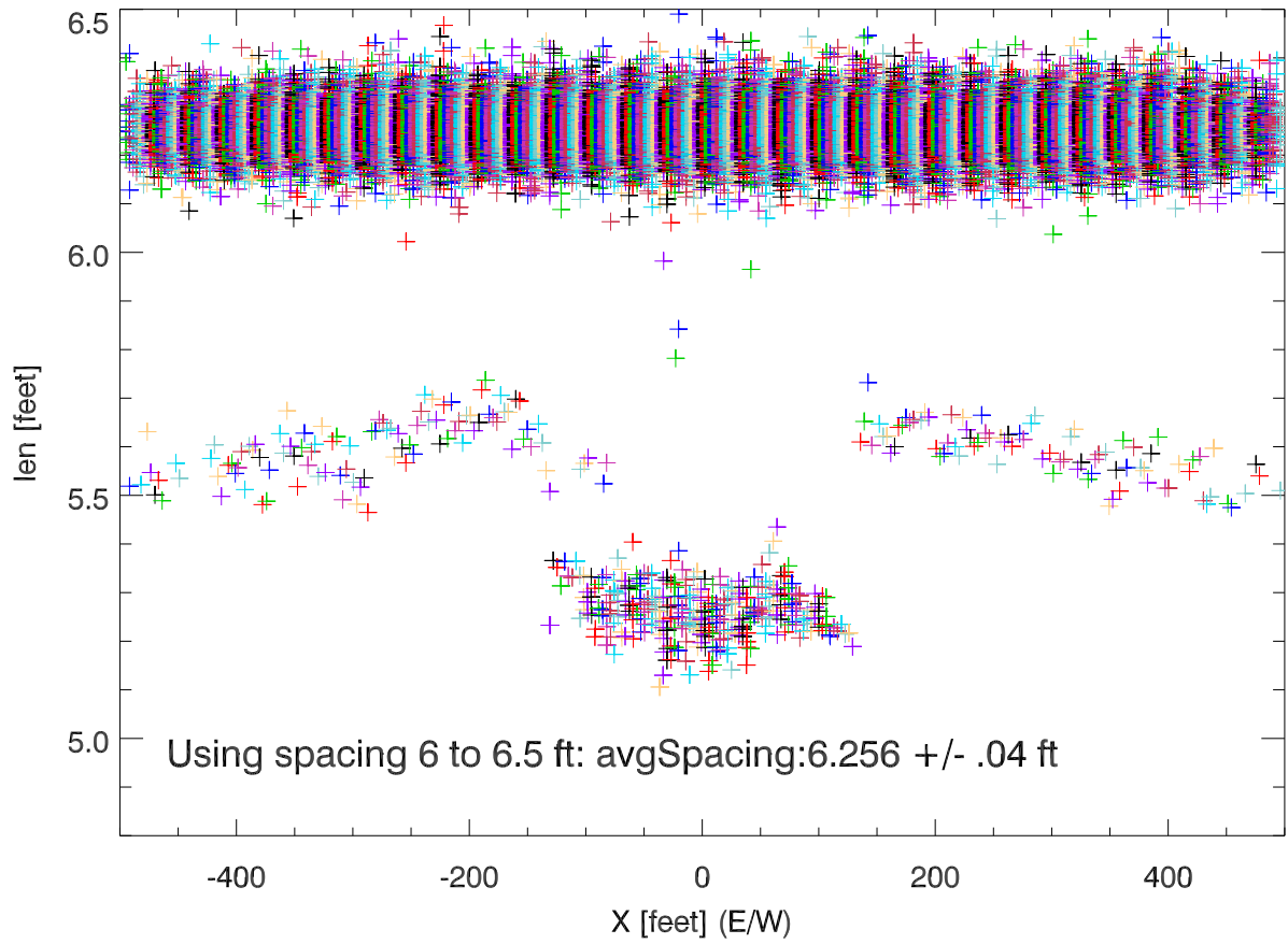
Long panel direction measured spacing vs X location (East/West)
