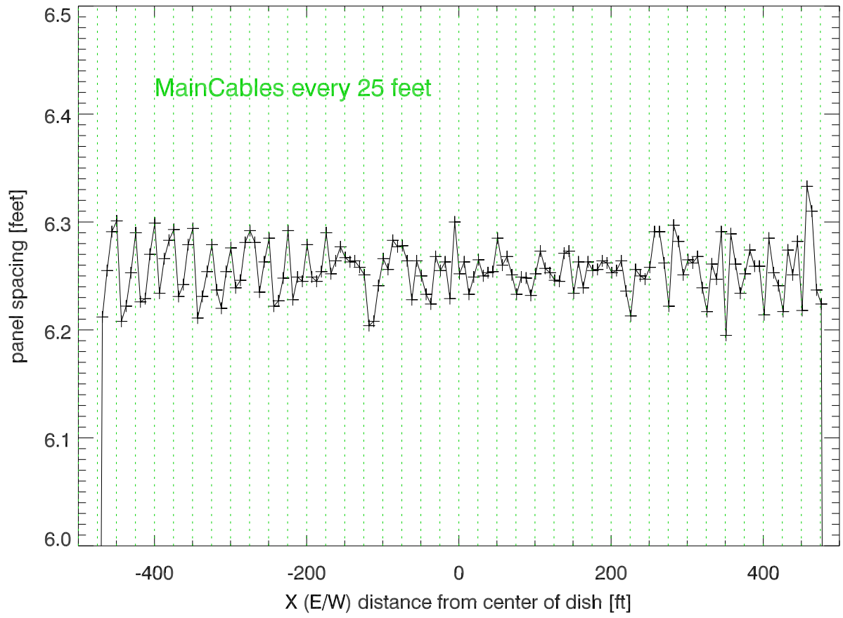
E/W panel spacing using median of each N/S strip
