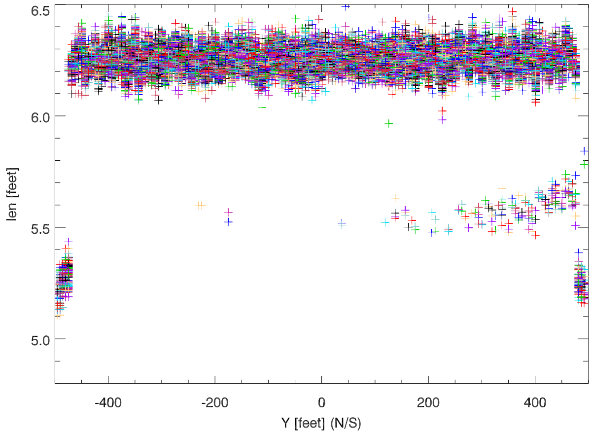
Long panel direction measured spacing vs Y location (North/South)
