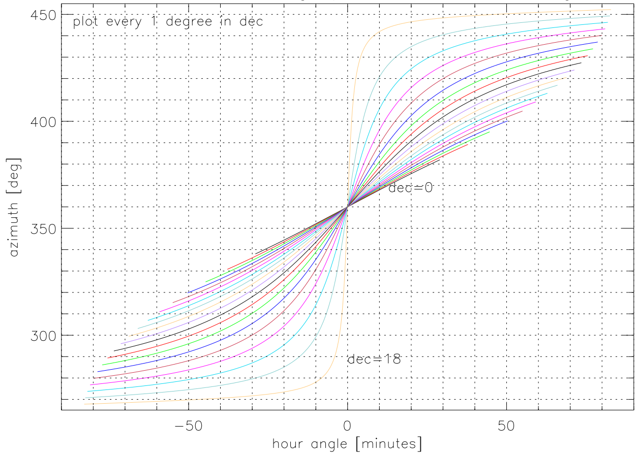
azimuth vs hour angle plotted for decs 0–18 deg
