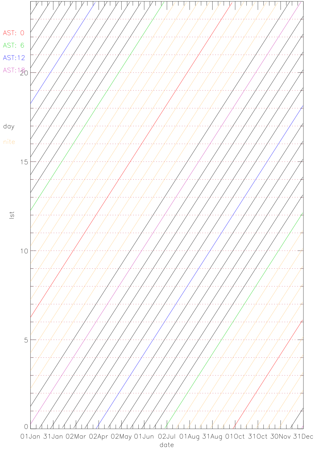
LST vs Date by Asthour for 2006
