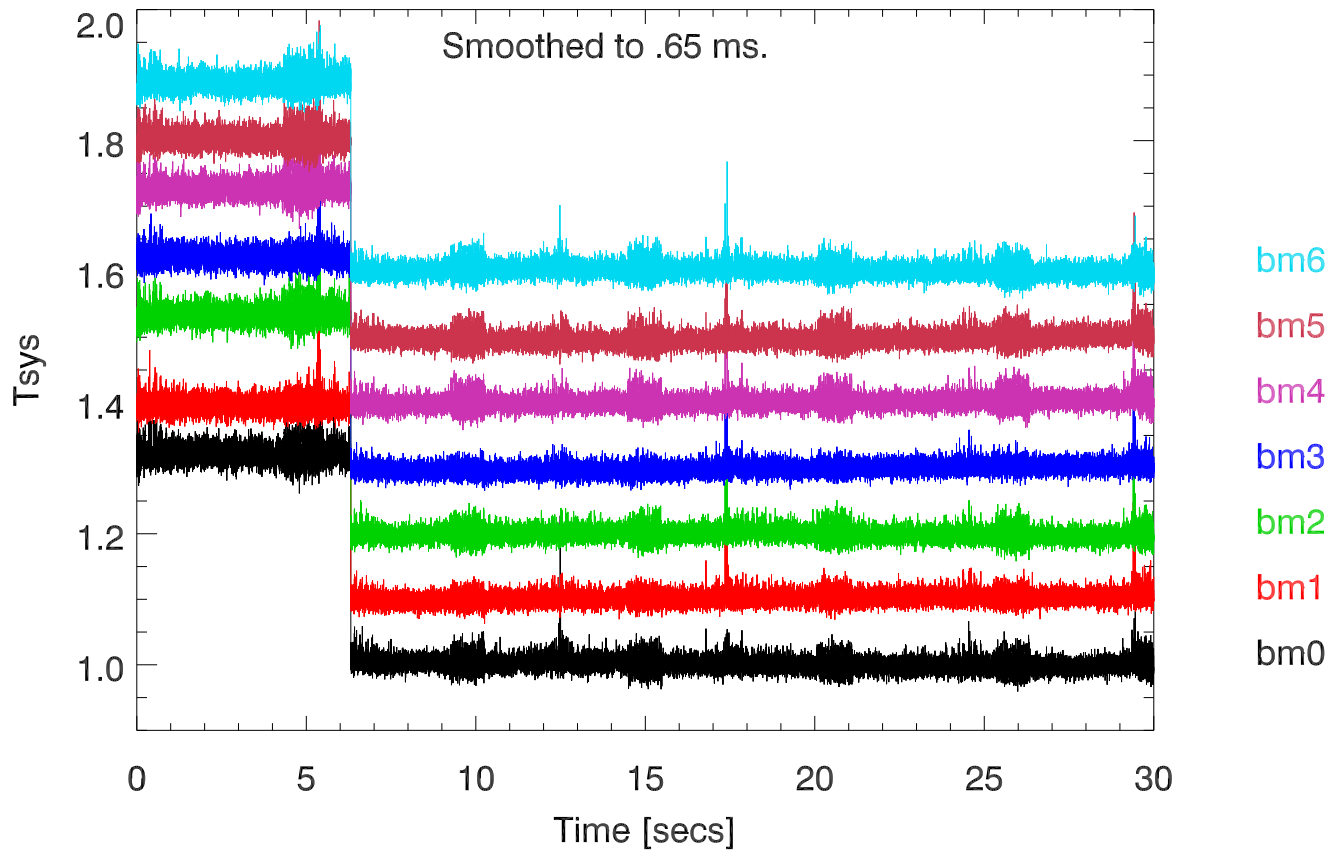
24may12 J1910+1017 TotalPwr(172Mhz) vs Time. 1300Mhz band
