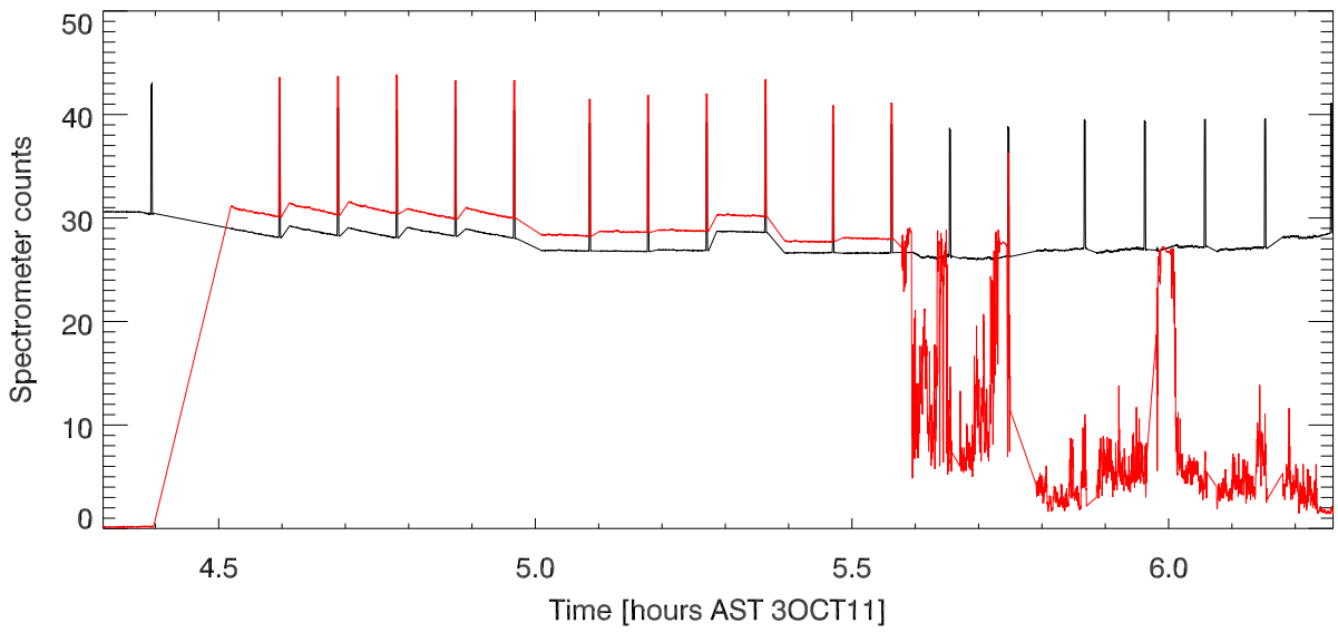
total pwr Tsys vs time. alfa bm6
