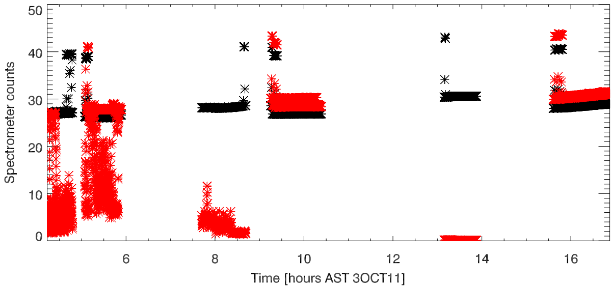
total pwr Tsys vs za. alfa bm6
