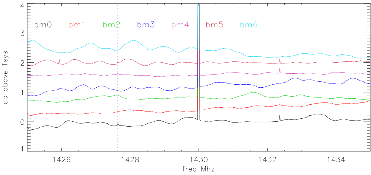
sinewave and 2.37 Mhz sidelobes PolB
