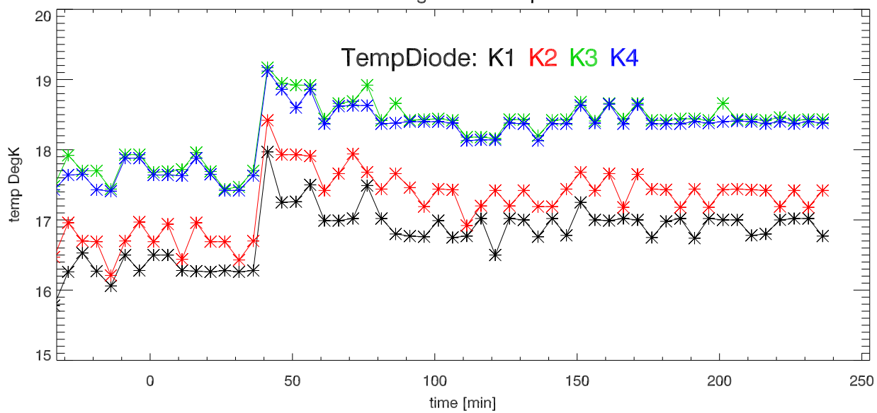
Alfa 20k Stage dewar temperatures
