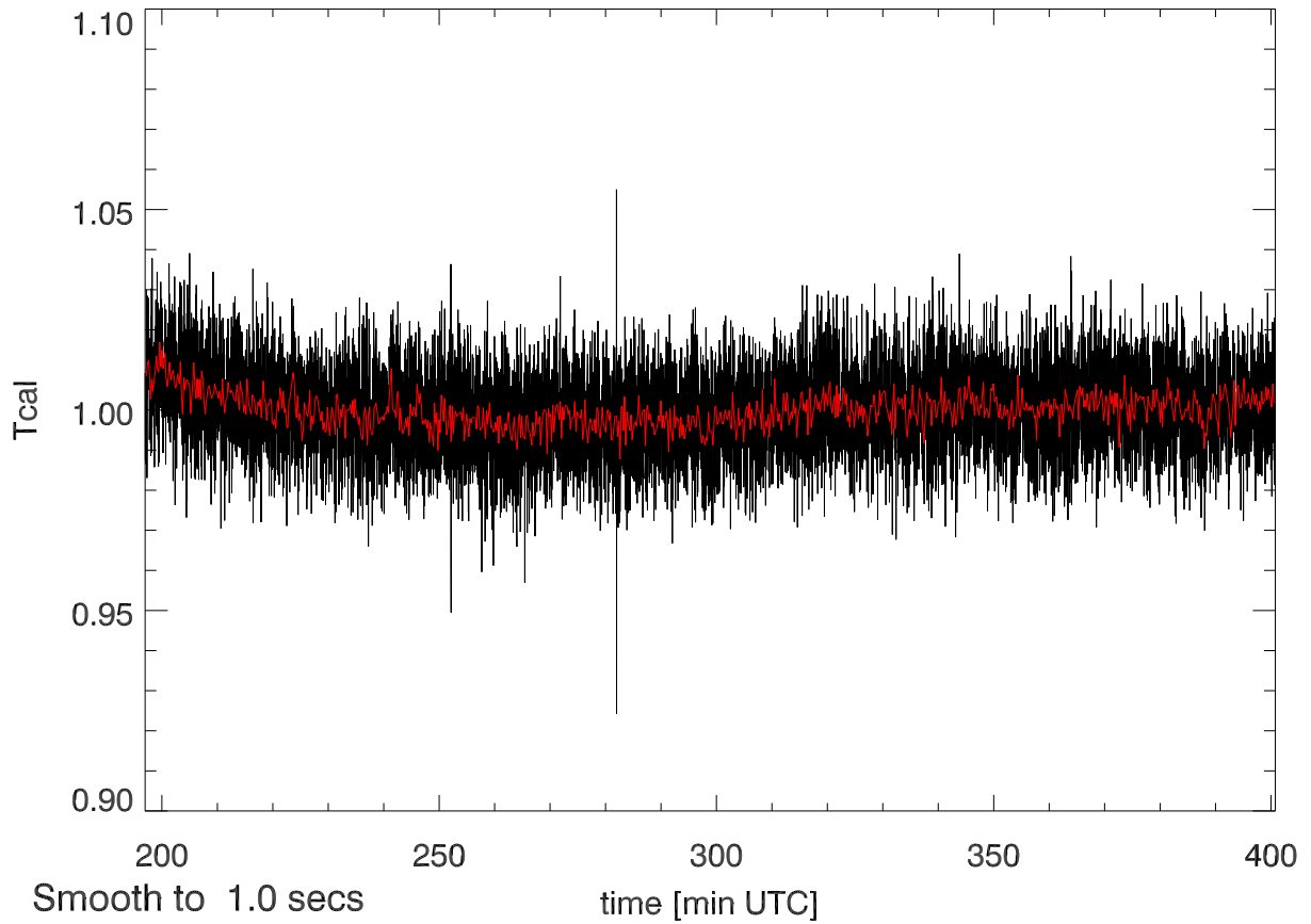
25aug13 calOn - calOff Beam6A SigA: 0.019
