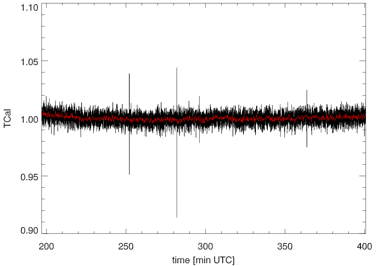
calOn - calOff Beam6B SigB: 0.008
