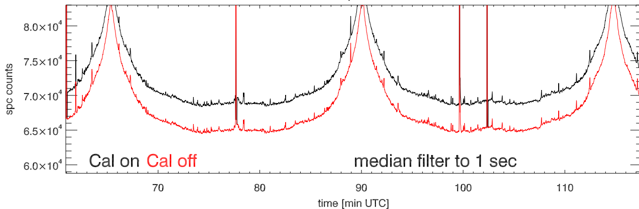
27dec15 a2030 tp vs time. Beam4A
