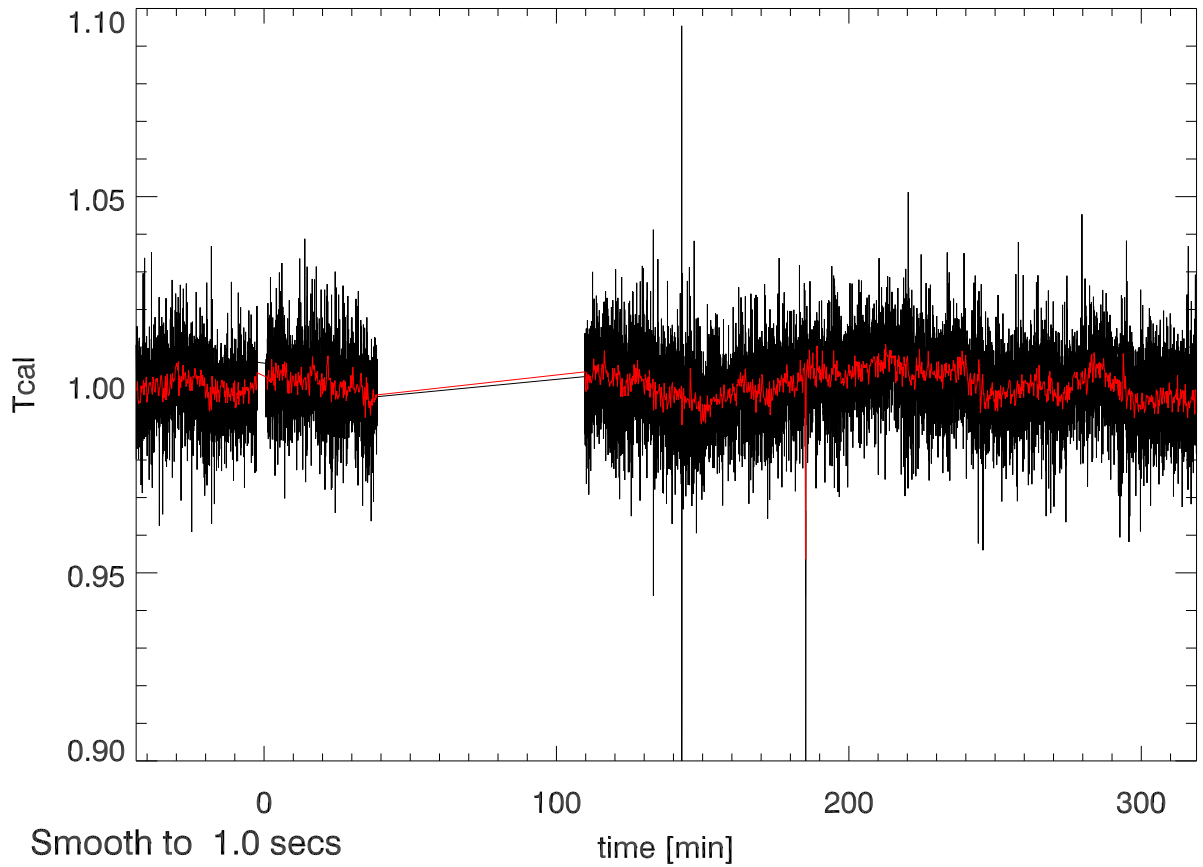
22jun12 calOn - calOff Beam4A SigA: 0.015
