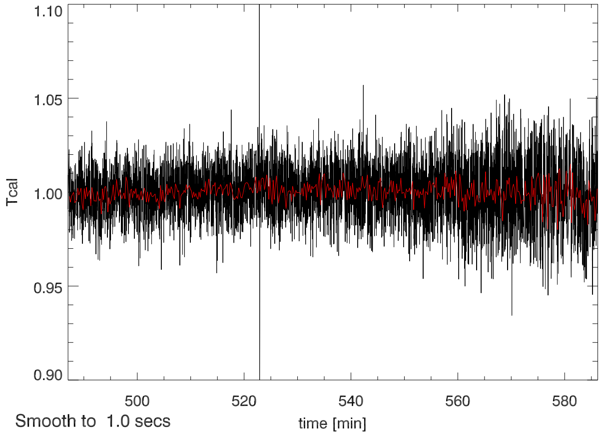
11nov11 calOn - calOff Beam4A SigA: 0.026
