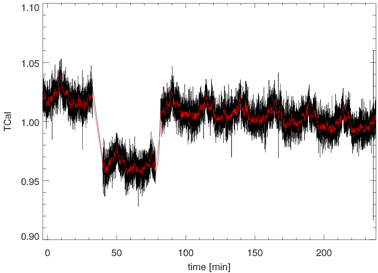
calOn - calOff Beam2B SigB: 0.023
