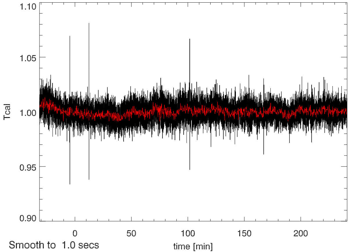
23may11 calOn - calOff Beam1A SigA: 0.014
