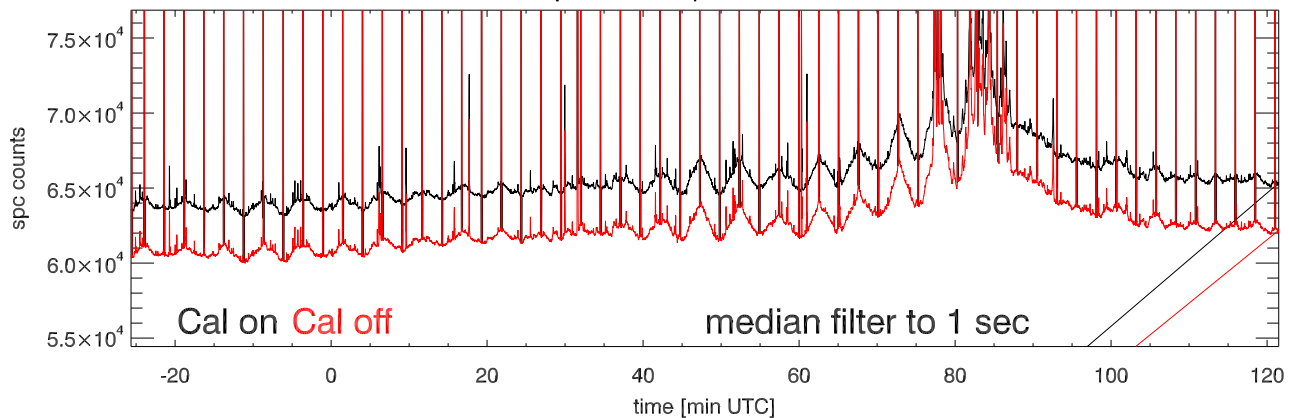
09sep13 a2030 tp vs time. Beam1A
