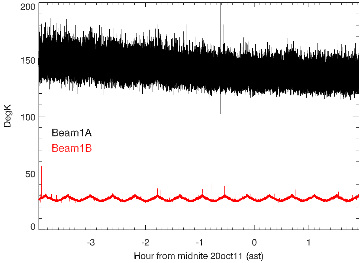
19oct11 a2130 alfa Tsys vs hour for Beam 1A,1B
