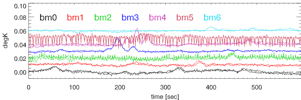
110214 Alfa totalPwr vs time. Scan:104500001
