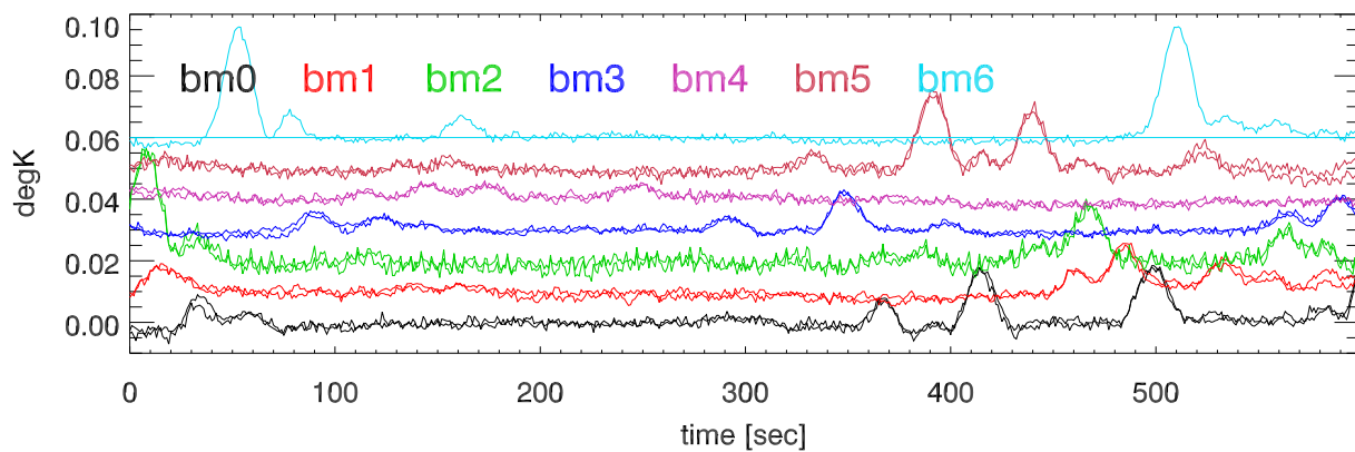
110131 Alfa totalPwr vs time. Scan:103100026
