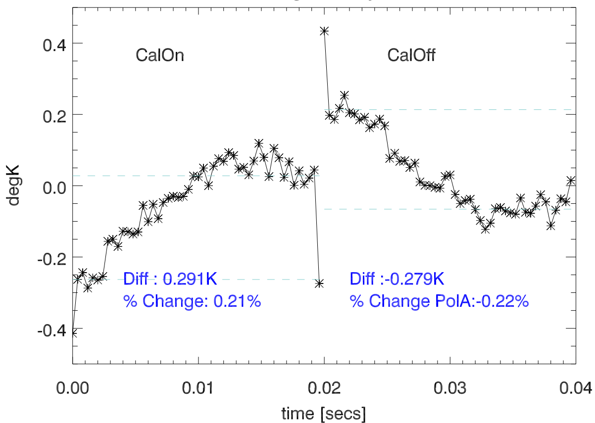
Differential change in Tsys calOn,calOff
