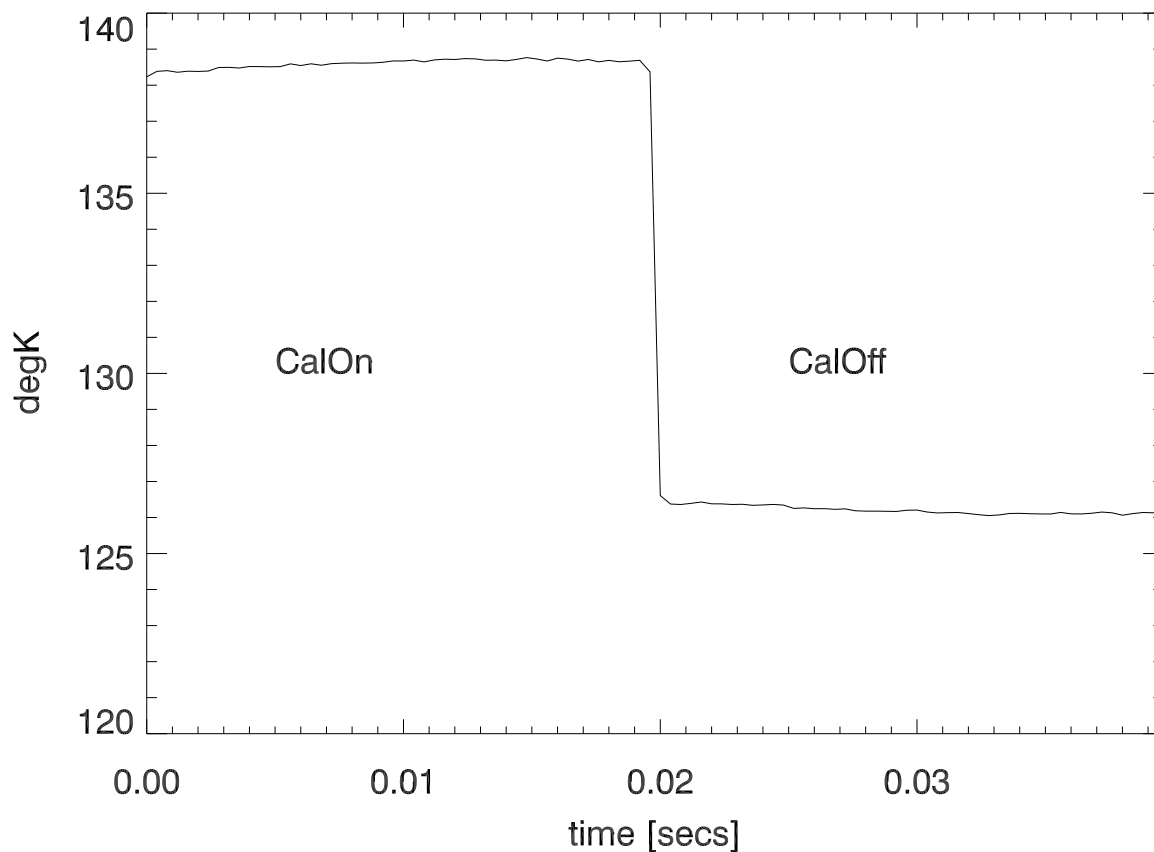
21dec13 10 sec folded winking cal on 3C138
