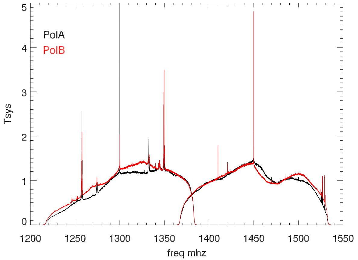
06jan14, alfa uncalibrated bandpass
