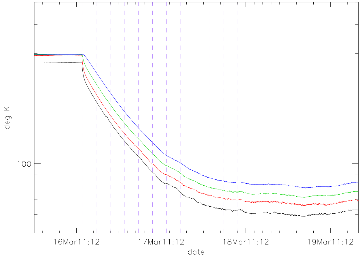
Dewar temps – 70K stage (year 2011) Alfa cooldown
