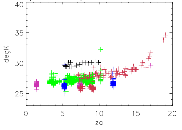
may05 Alfa Tsys vs za Pixel 5 Pol B
