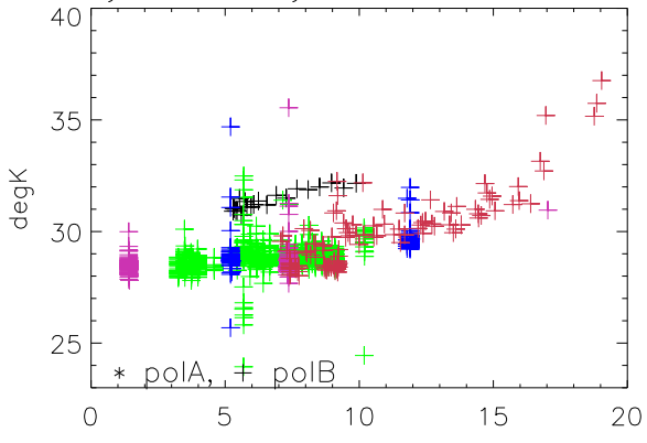
may05 Alfa Tsys vs za Pixel 0 Pol A
