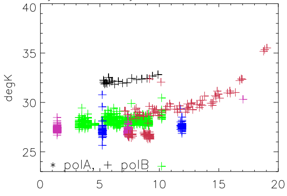
may05 Alfa Tsys vs za Pixel 4 Pol A
