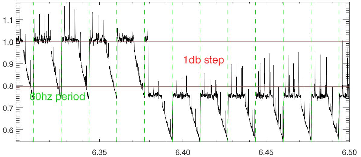
blowup.. normalize to cal on
