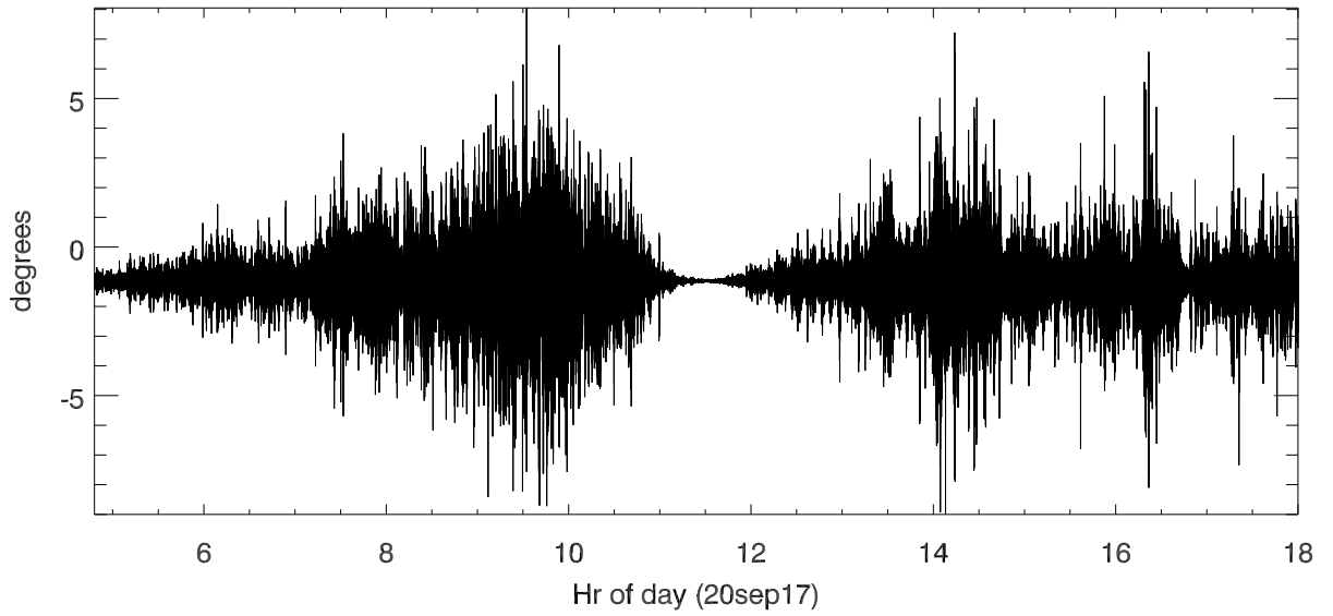
20sep17 pitch tilt sensor vs hour of day
