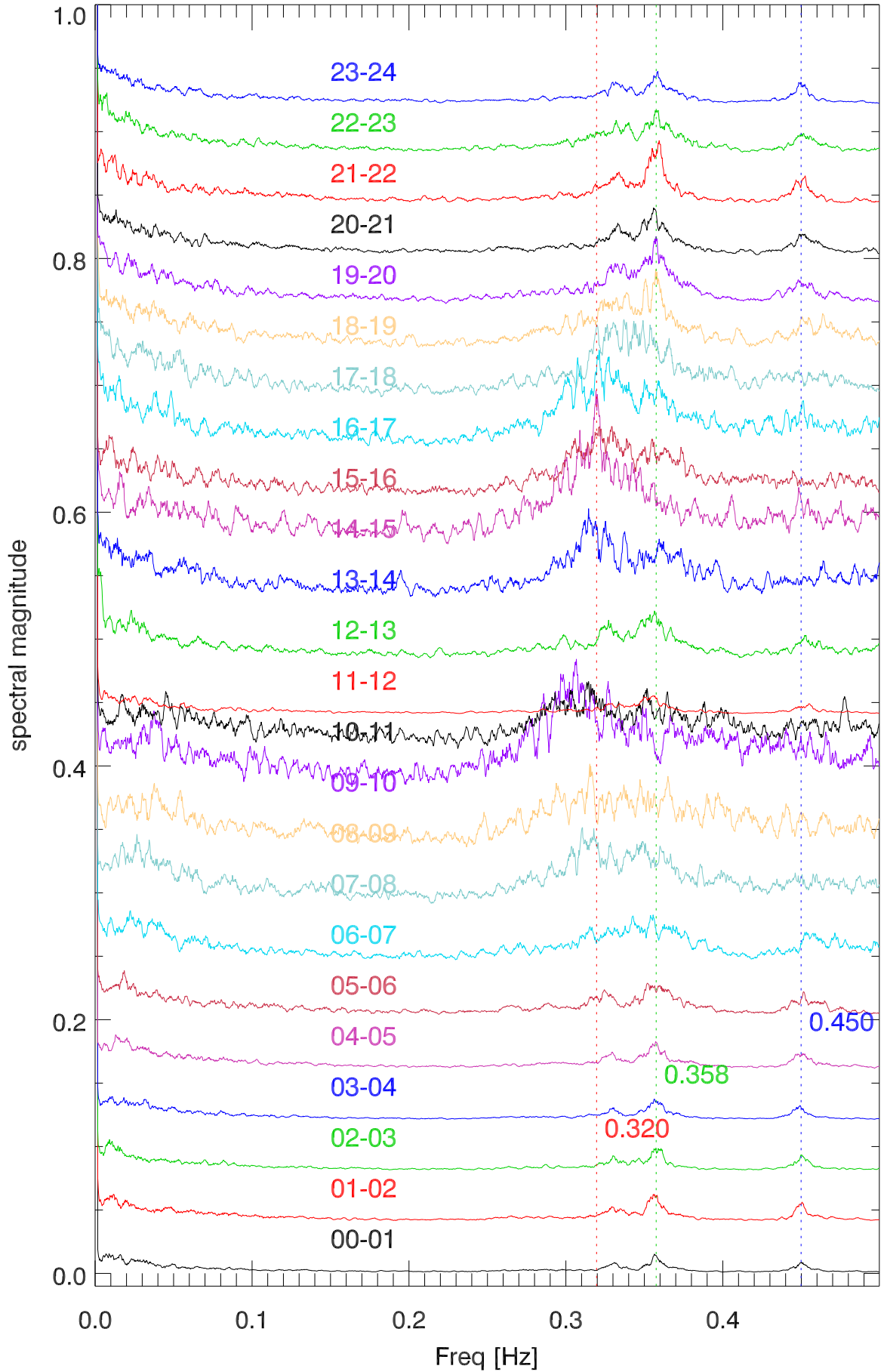
20sep17 spectra of tiedown tension by hour of day
