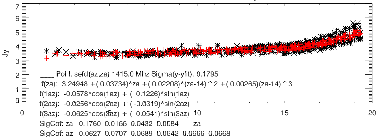
lbw 1415 sefd vs za and fit dec17-jun18
