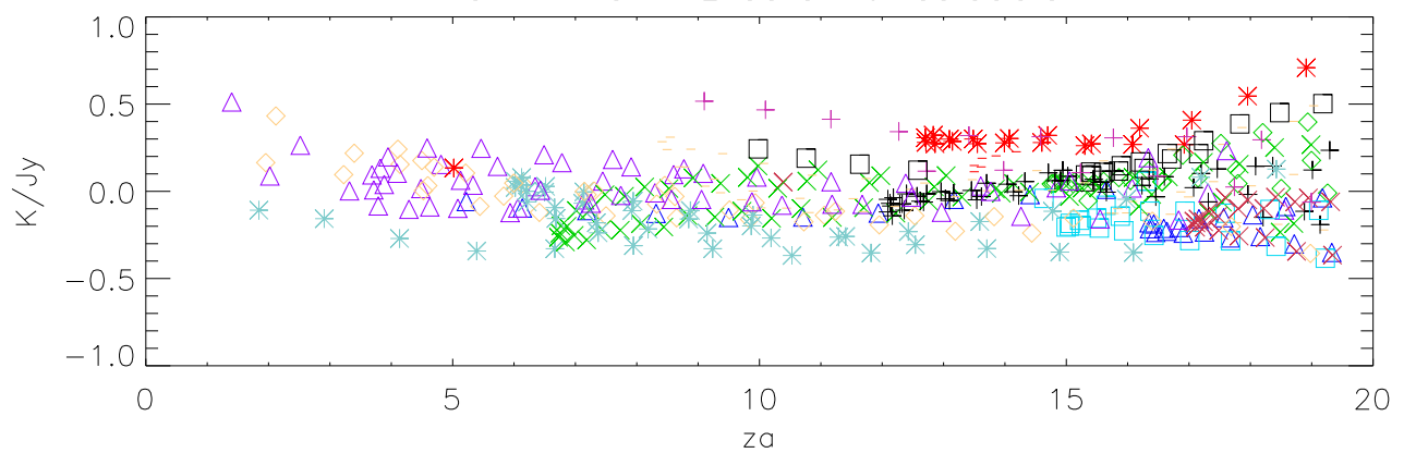
lbw 1415 Mhz sefd fit residuals
