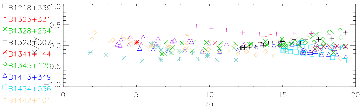
lbw 1375 Mhz sefd fit residuals
