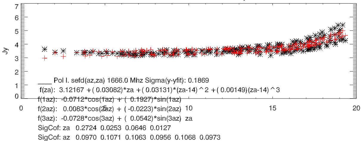
lbw 1666 sefd vs za and fit dec17-jun18
