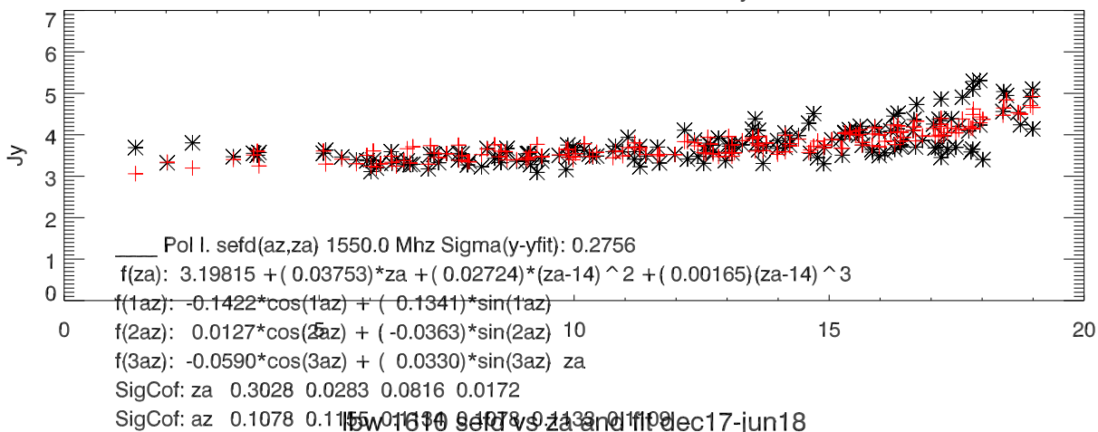
lbw 1550 sefd vs za and fit dec17-jun18
