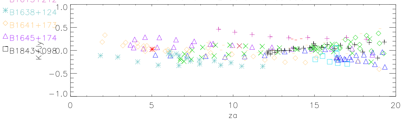
lbw 1415 Mhz sefd fit residuals
