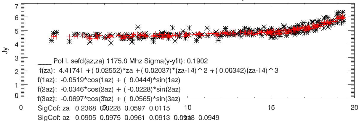
lbw 1175 sefd vs za and fit dec17-jun18
