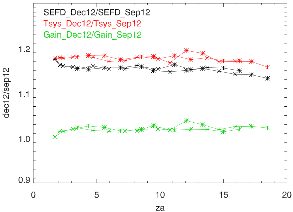
SEFD, Tsys, Gain ratios dec12/sep12
