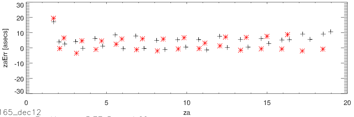
10dec12 lbw 1415 MHz.compare 3C138: Dec12 and Sep09 za error vs za
