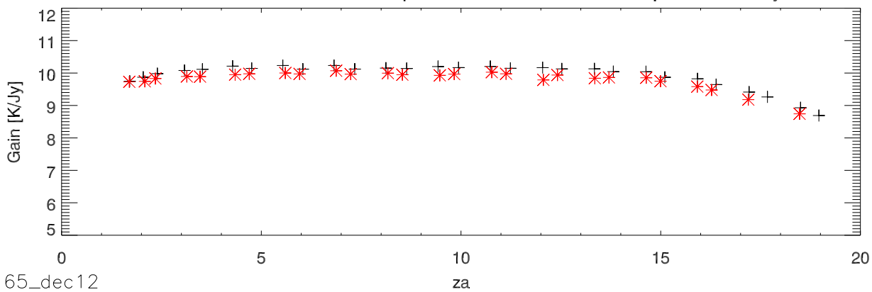
10dec12 lbw 1415 MHz.compare 3C138: Dec12 and Sep09 Gain K/Jy
