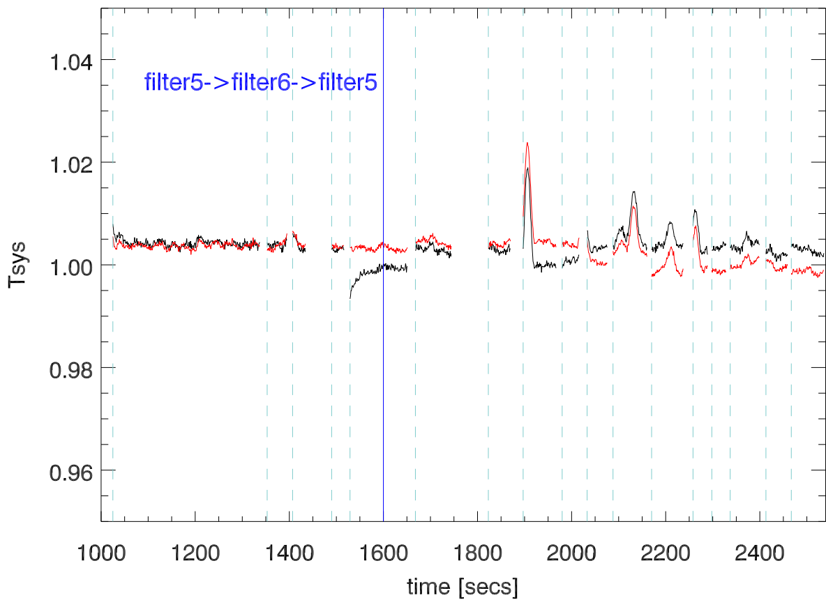
TestOtherFitlers. filter5->filterN->filter5
