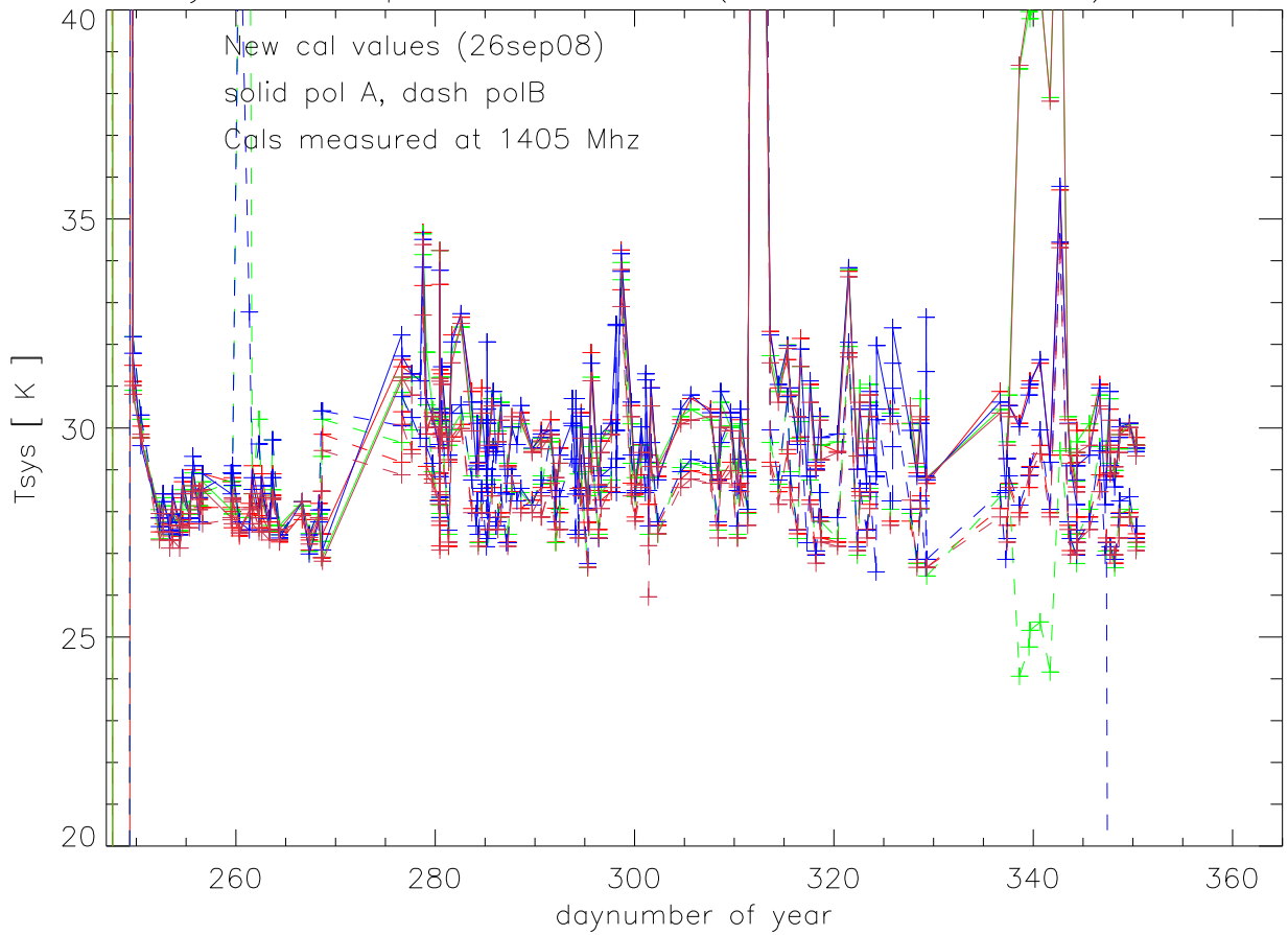
system temperature for LBW (receiver number R5) 2008
