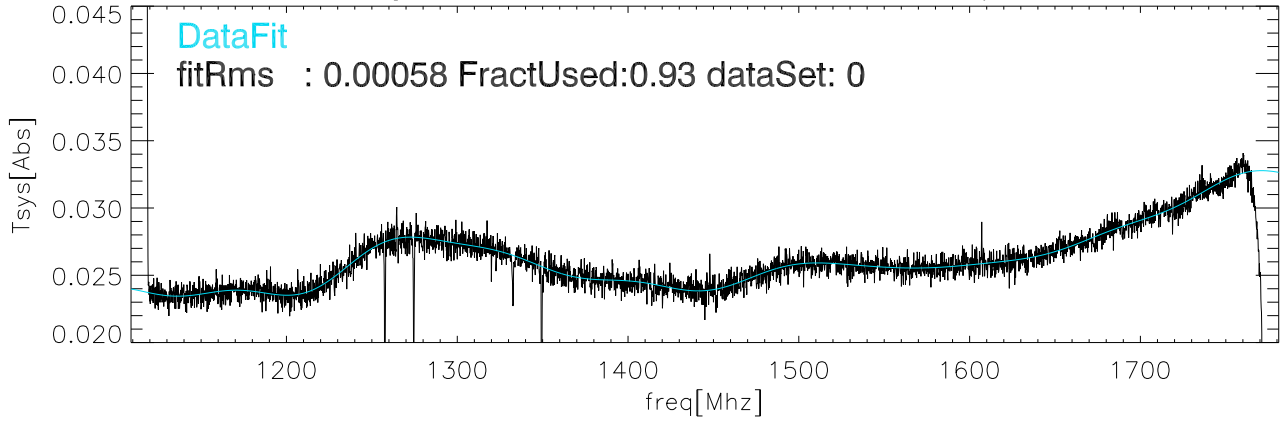
28apr16 Averaged data and fit for CalDeFlection/Tsys on abs polB
