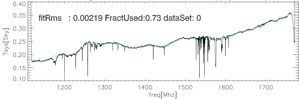
28apr16 Averaged data and fit for CalDeFlection/Tsys on Sky polB
