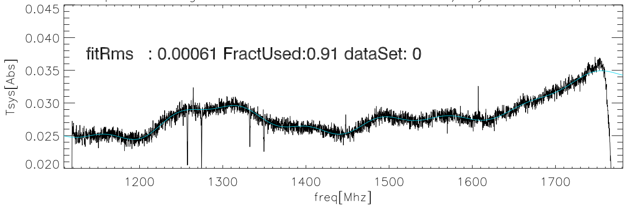
28apr16 Averaged data and fit for CalDeFlection/Tsys on Sky polA
