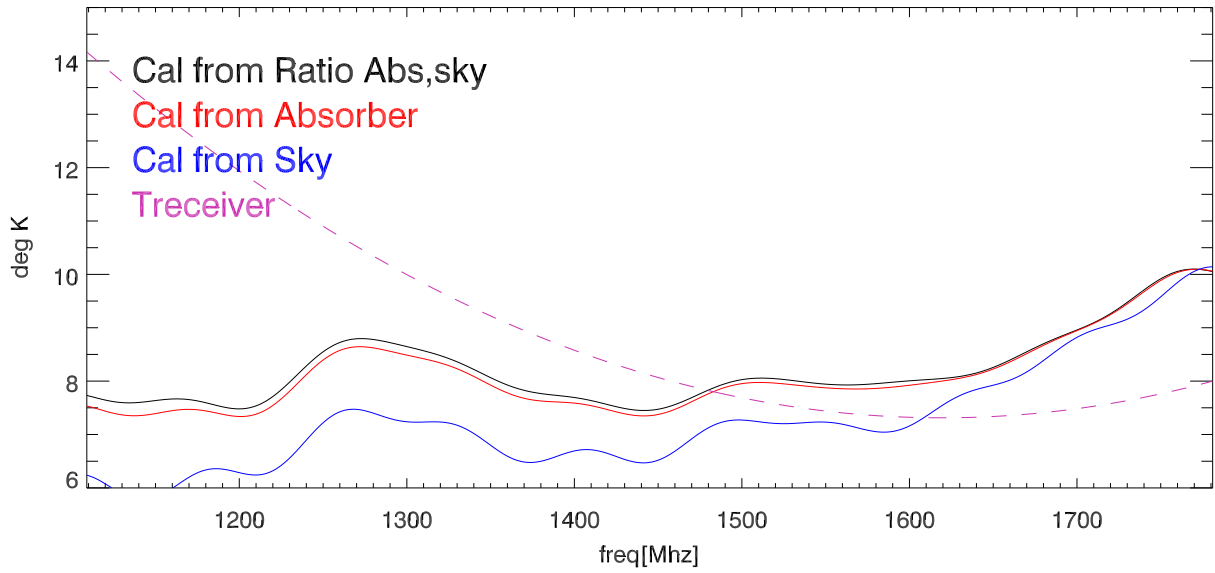
28apr16Cal in Kelvins vs freq polA
