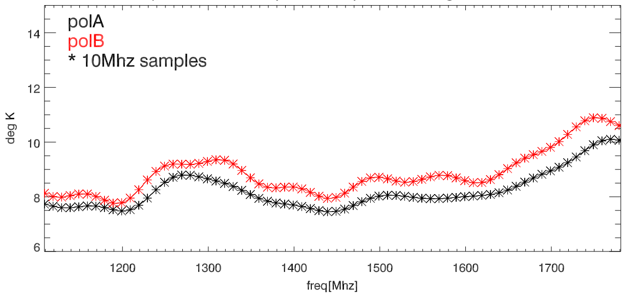
28apr16Cal in Kelvins polA,B overplotted, Average dataset fits
