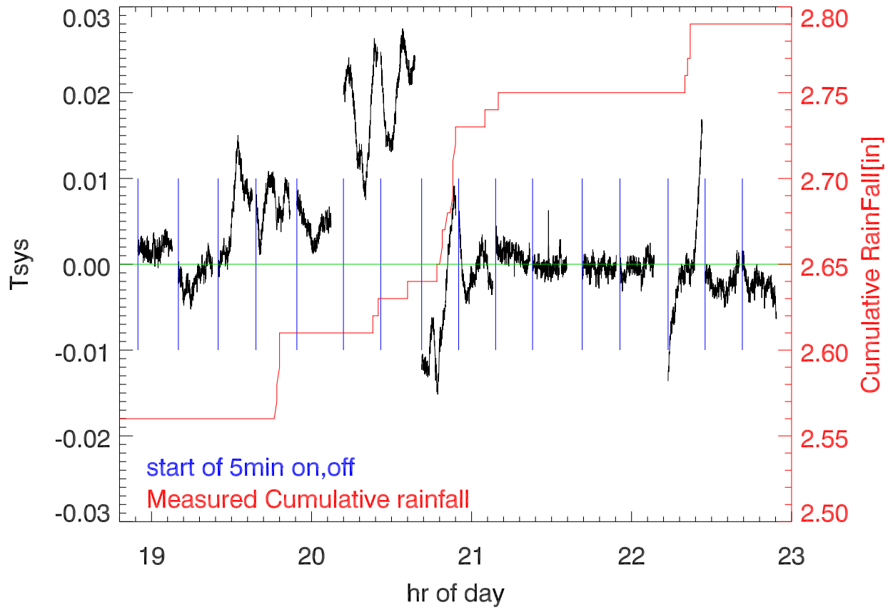
14apr12 a2335 lbw: totalPwr on/off-1 vs hour during rain.
