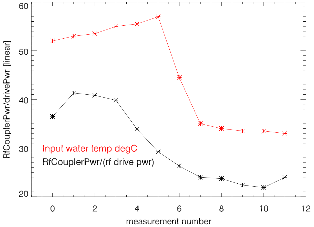
08may15:TX 4 gain variation
