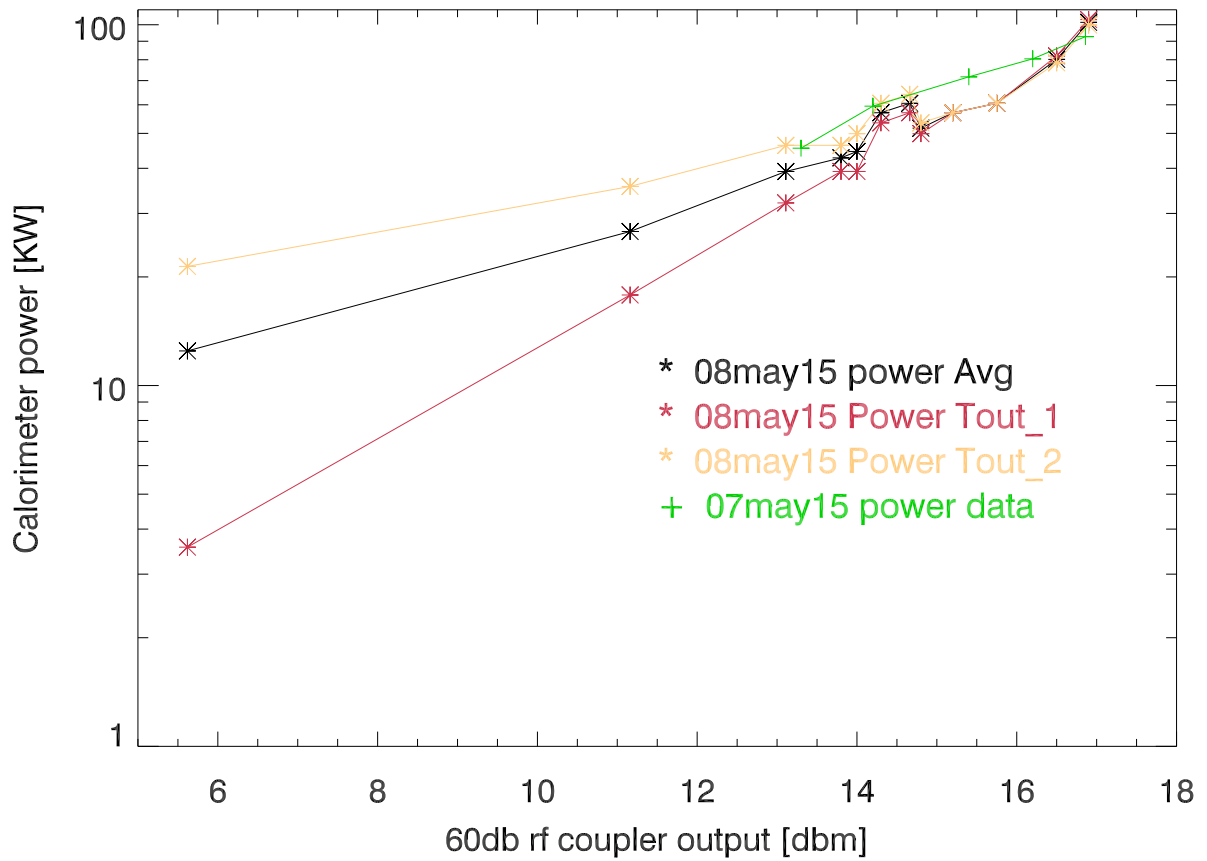
08may14 pwr using 1st,2nd,and avg output water temp
