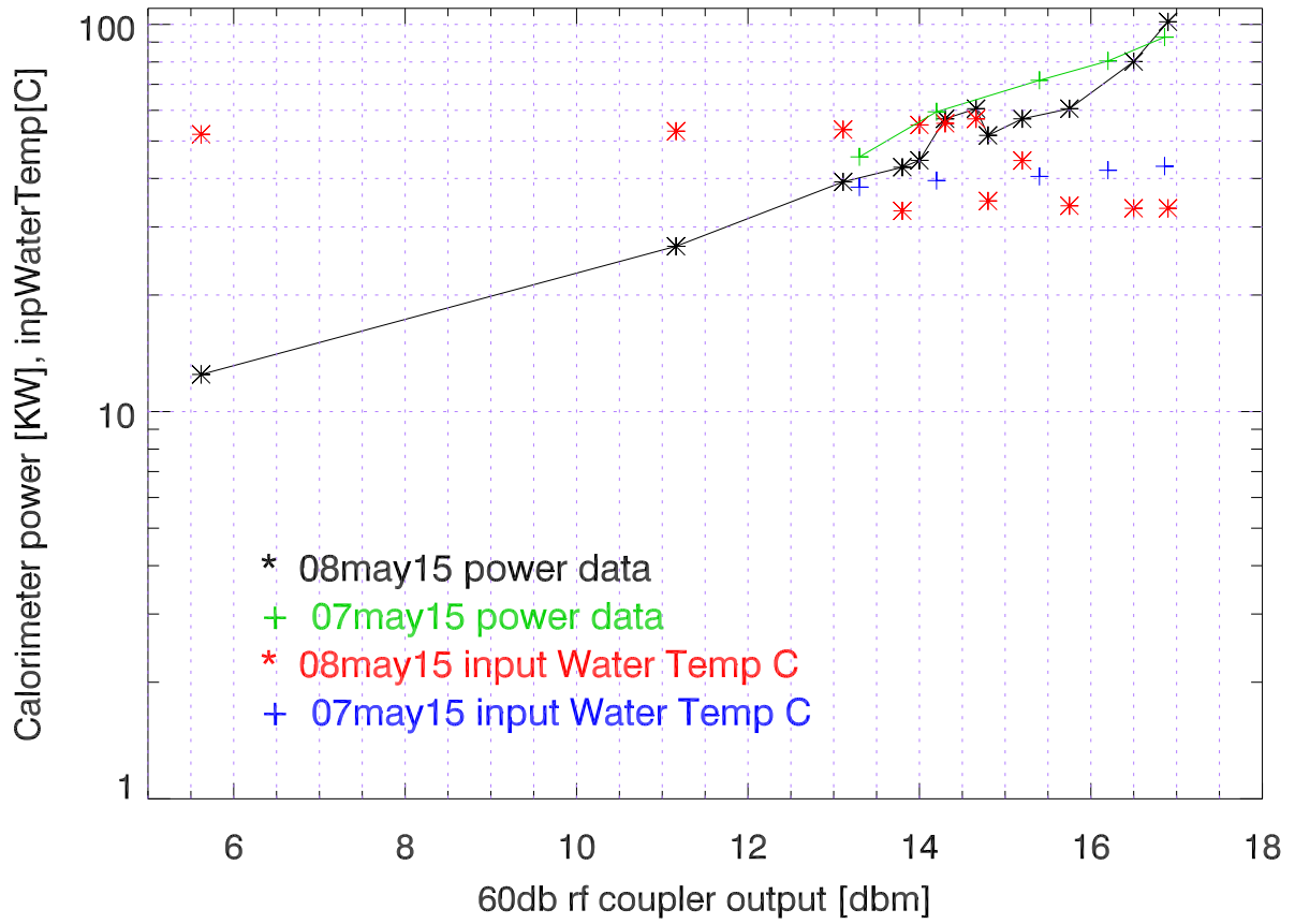
Tx4 calorimeter vs rf Coupler output
