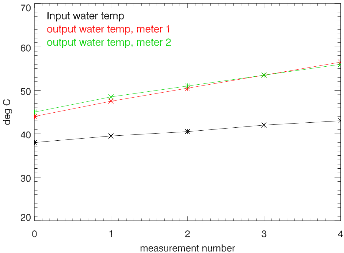
07may15:Water temps for Calorimeter
