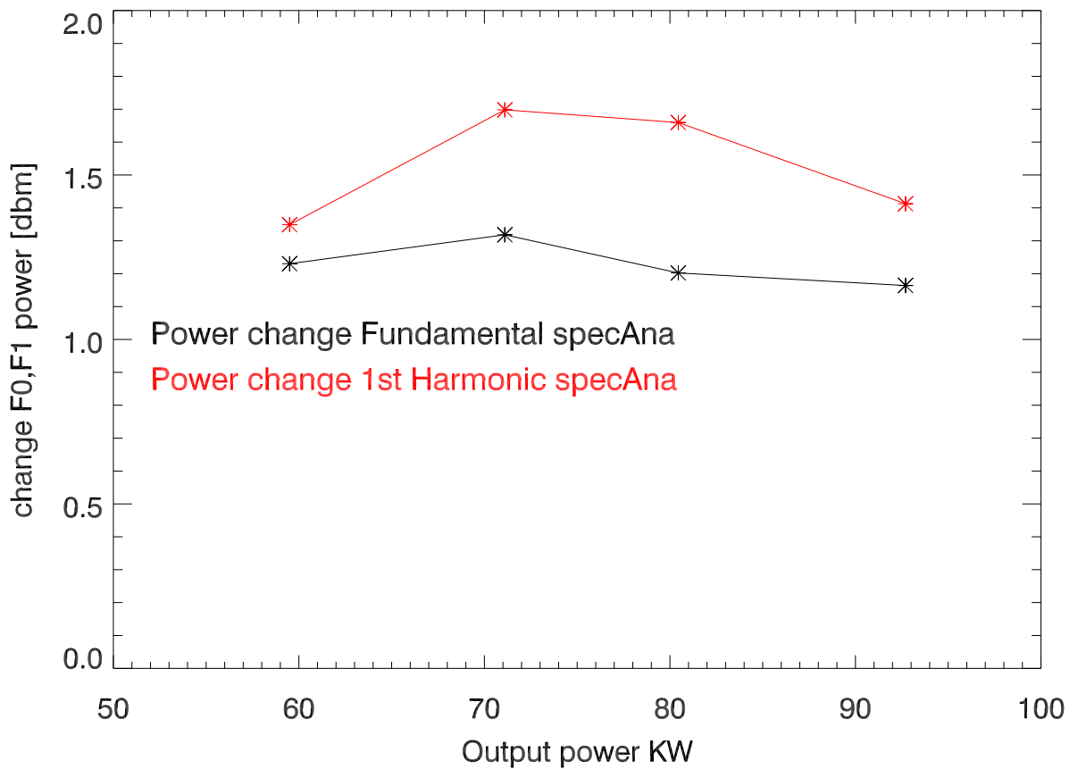
Delta power fundamental and 1st harmonic
