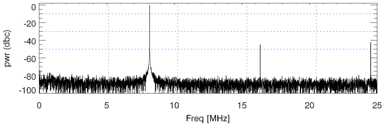
170223 tx4 tube monitor ports: spectral density. BroadBand
