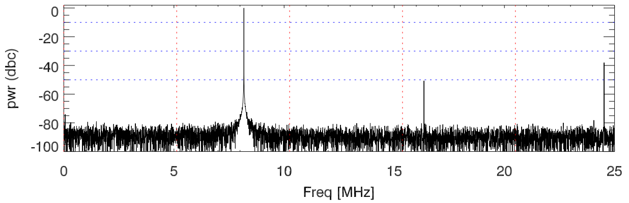
170223 tx2 tube monitor ports: spectral density. BroadBand
