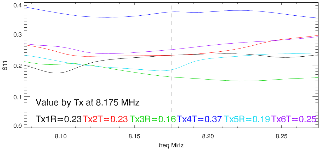
31aug16 HF 8 MHz dipoles S11 vs freq. Mesh at 5MHz Position
