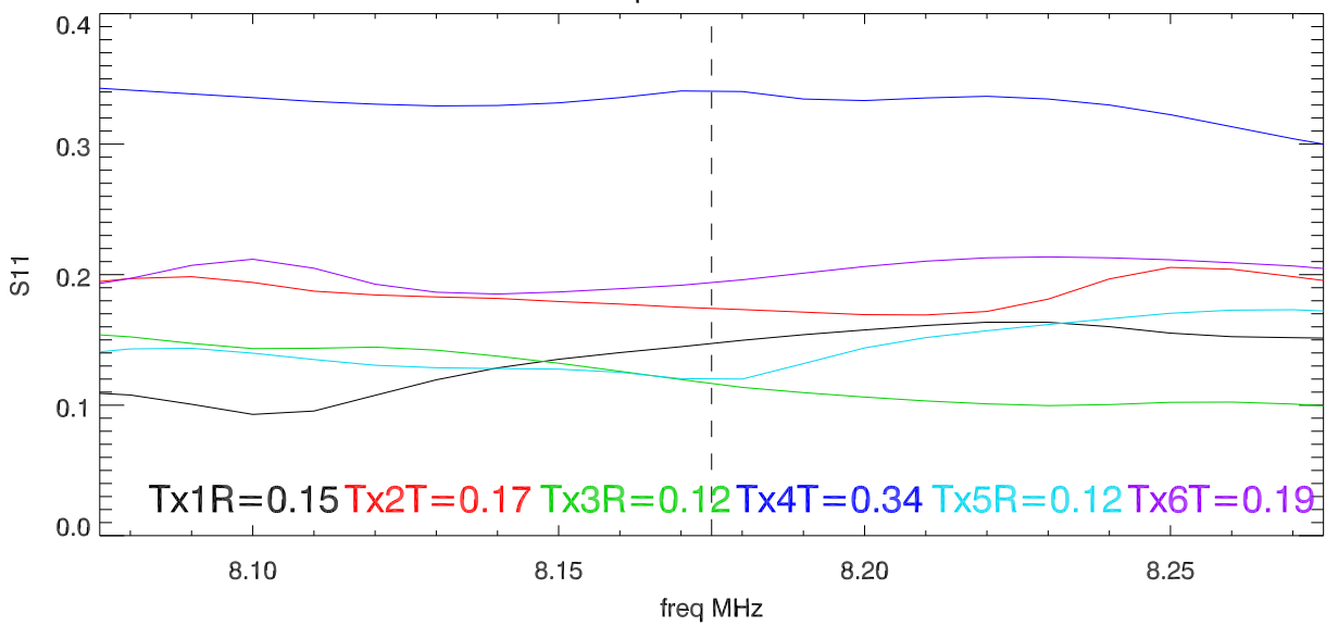
S11 vs freq. Mesh at 5MHz - 10ft
