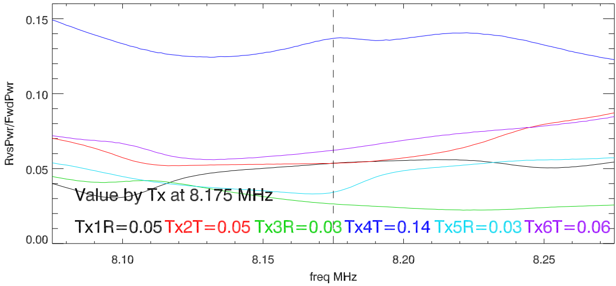
31aug16 HF 8 MHz dipoles RvsPwr/FwdPwr vs freq. Mesh at 5MHz Position
