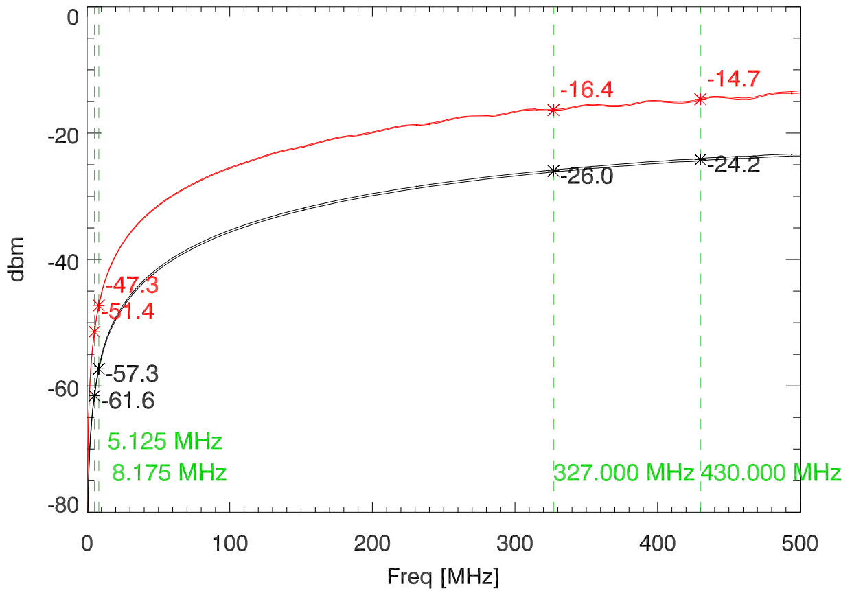
06may15 S21 HF rf coupler calibration
