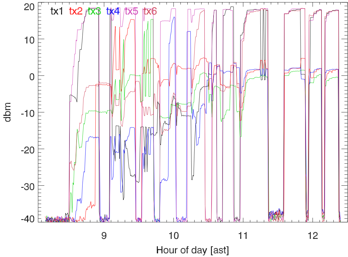
20sep16 8.175 Mhz tx power. rf coupler output
