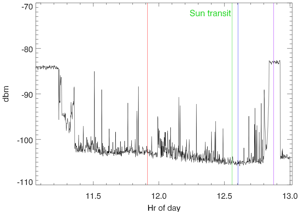
03jul18 average totPwr (100KHz about 8.175Mhz) vs hr of day
