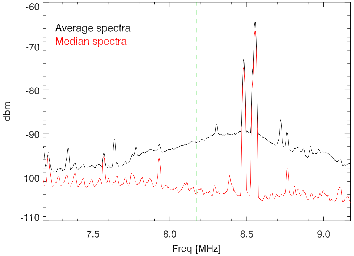
03aug18 average spectra. hf 8Mhz dipole 1. RBW=10KHz
