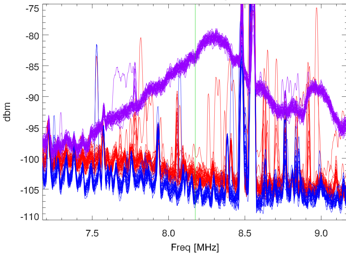
spectra from differing rfi areas
