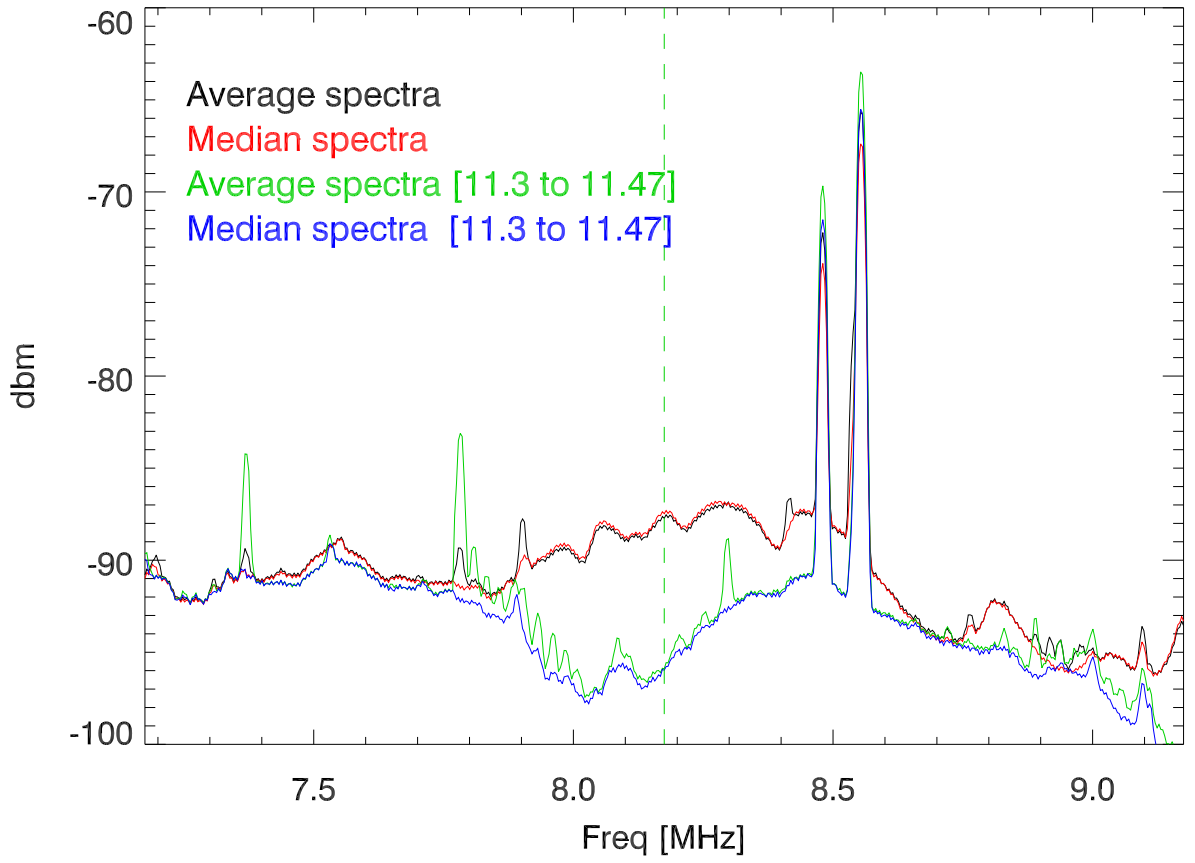
02aug18 average spectra. hf 8Mhz dipole 1. RBW=10KHz
