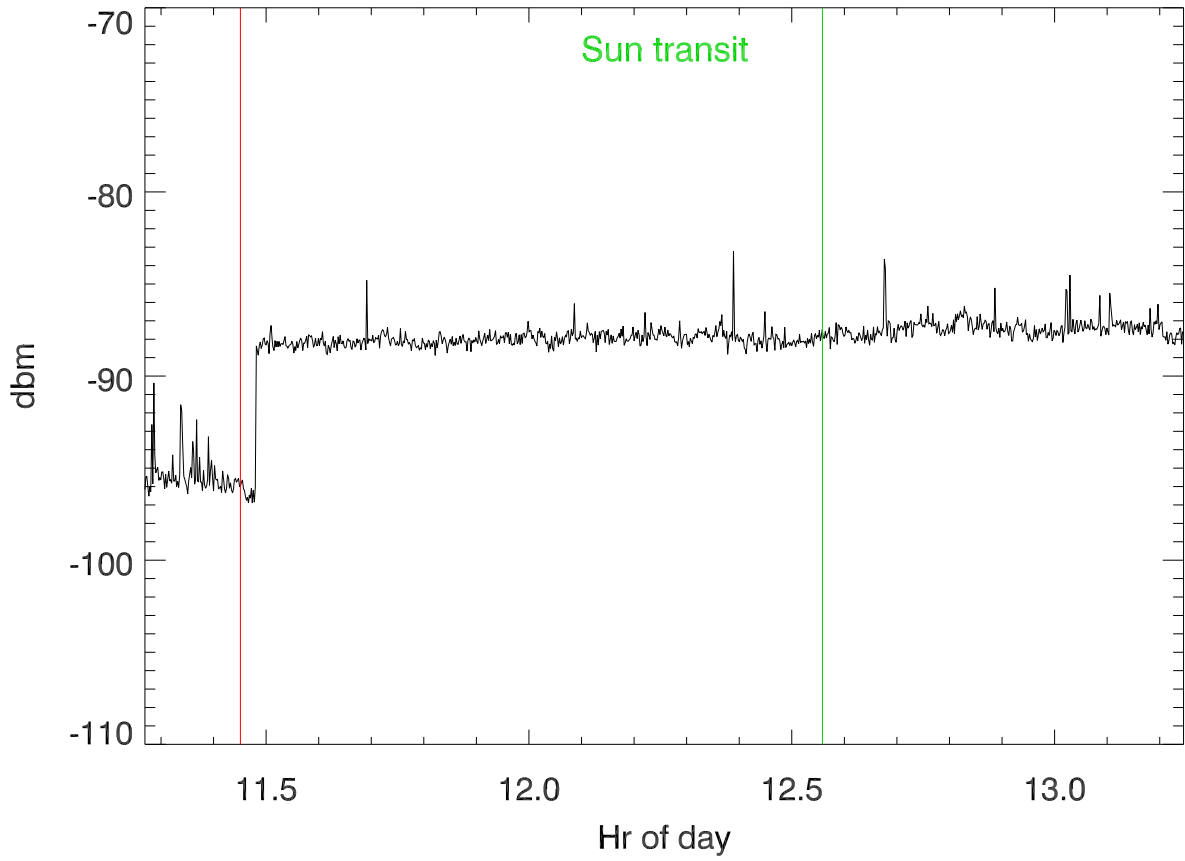
02aug18 average totPwr (100KHz about 8.175Mhz) vs hr of day
