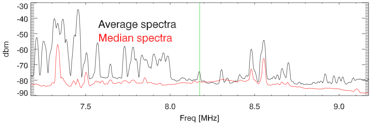
27jul18 average spectra. hf 8Mhz dipole 1. RBW=10KHz data:18.4 - 24.0
