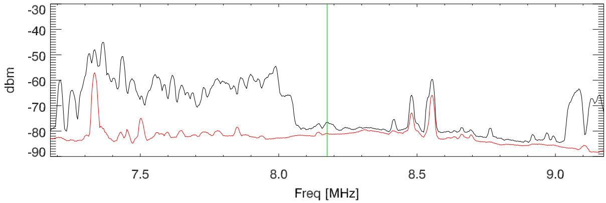
29jul18 average spectra. hf 8Mhz dipole 1. RBW=10KHz data: 0.0 - 24.0
