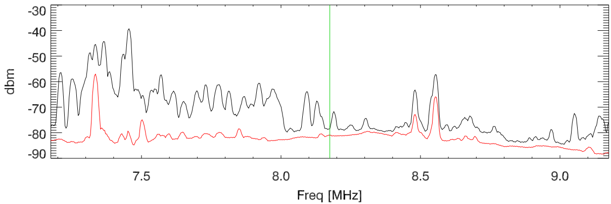
28jul18 average spectra. hf 8Mhz dipole 1. RBW=10KHz data: 0.0 - 24.0
