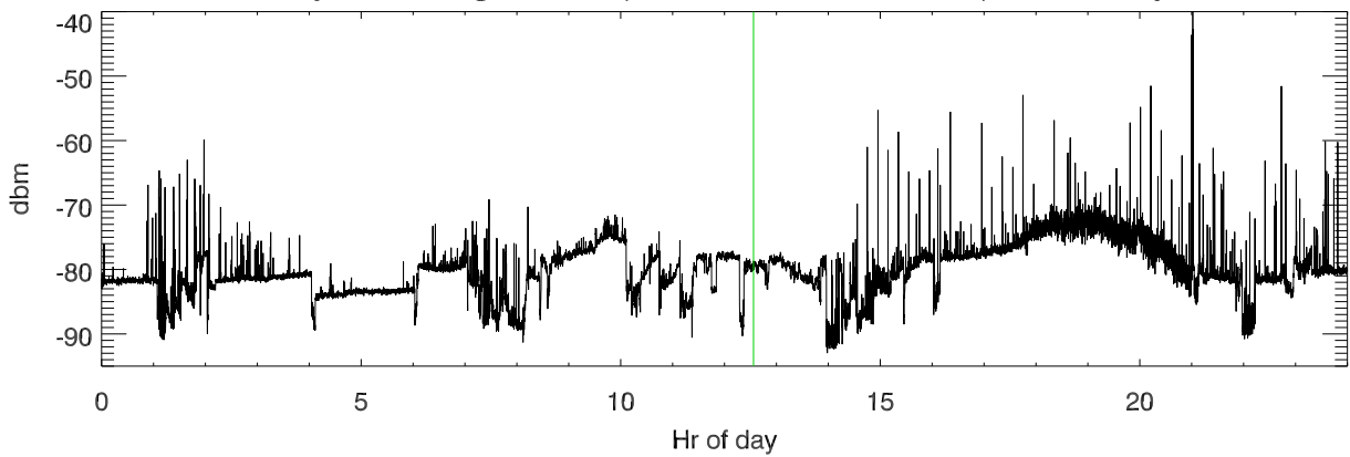
29jul18 average totPwr (100KHz about 8.175Mhz) vs hr of day
