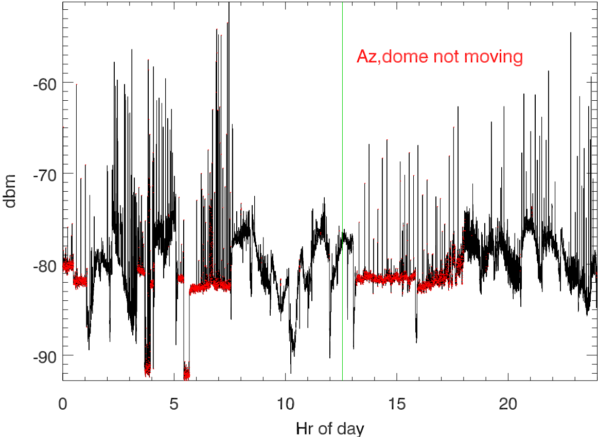
29jul18 average totPwr (100KHz about 8.175Mhz) vs hr of day
