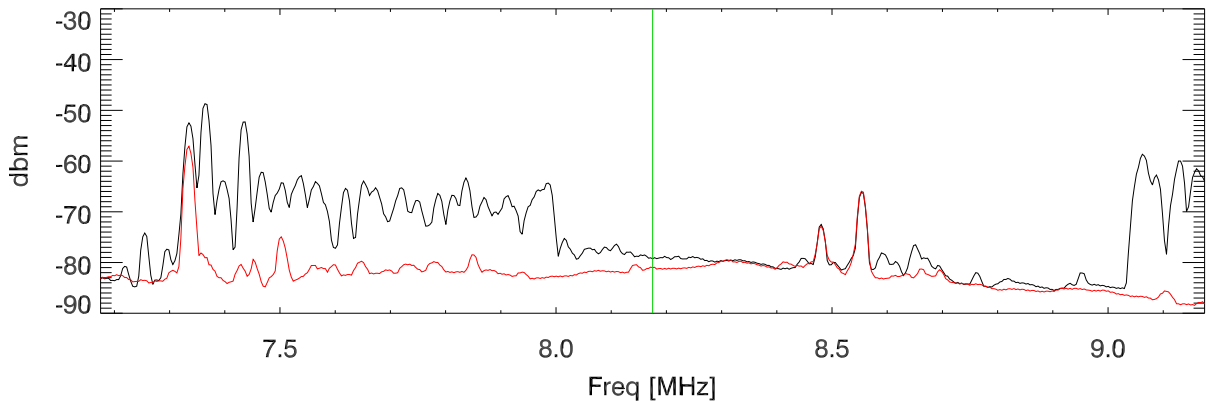
30jul18 average spectra. hf 8Mhz dipole 1. RBW=10KHz data: 0.0 - 8.4
