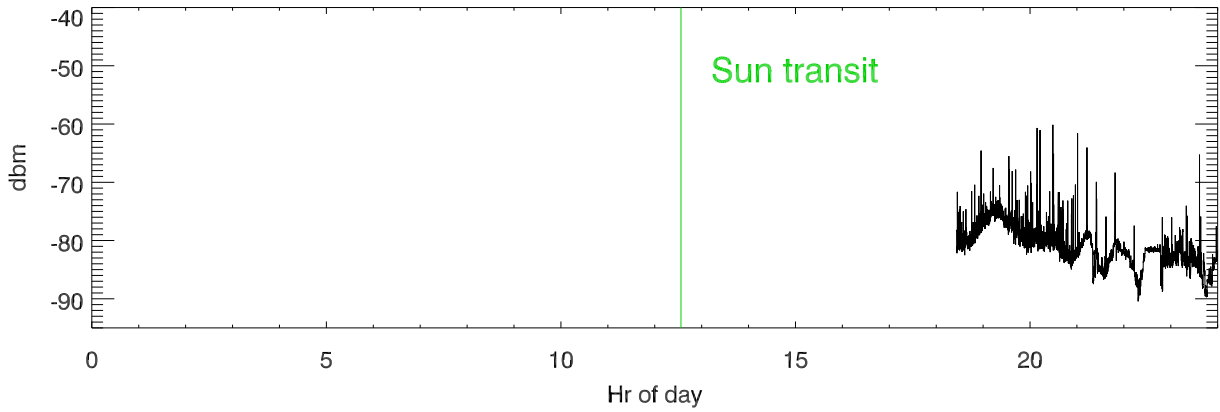
28jul18 average totPwr (100KHz about 8.175Mhz) vs hr of day
