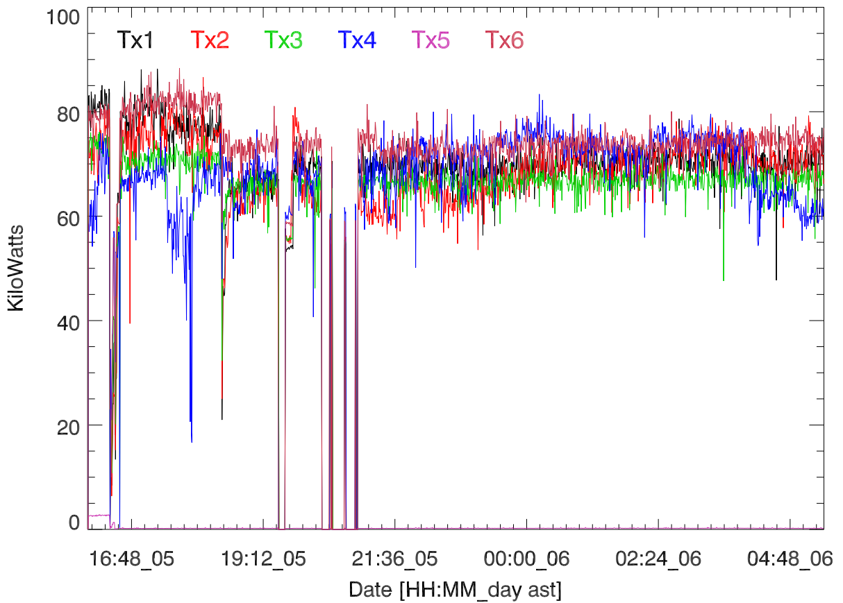
TxPwr by Tx. 05oct16:T2915. Salih Bostan
