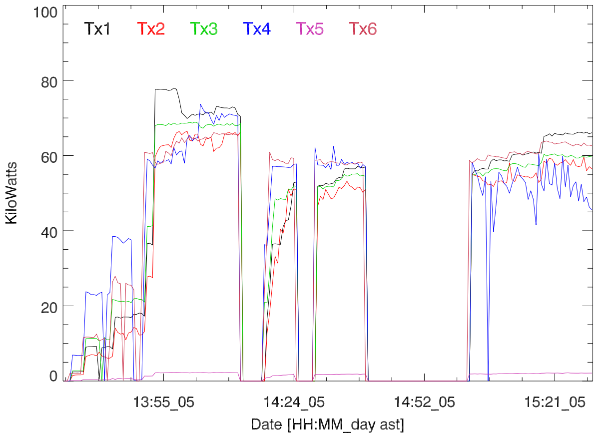
TxPwr by Tx. 05oct16:T2566. Paul BernHardt
